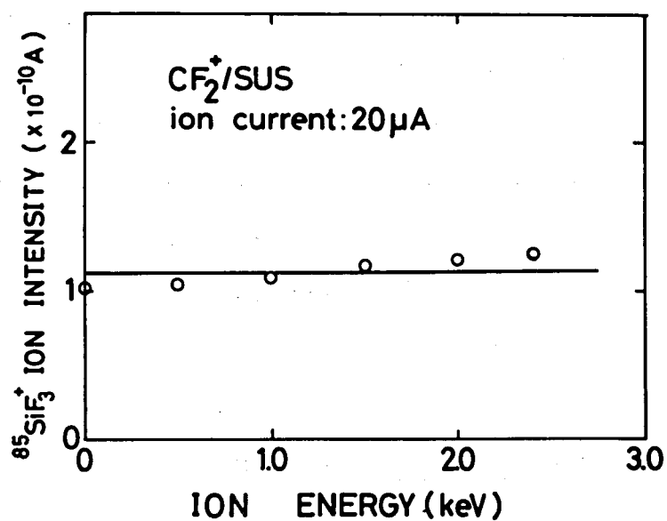
Fig. 4.5 Energy dependence of m/e=85 ion intensity for \text{CF}_2^+/\text{SUS} ion bombardment.
