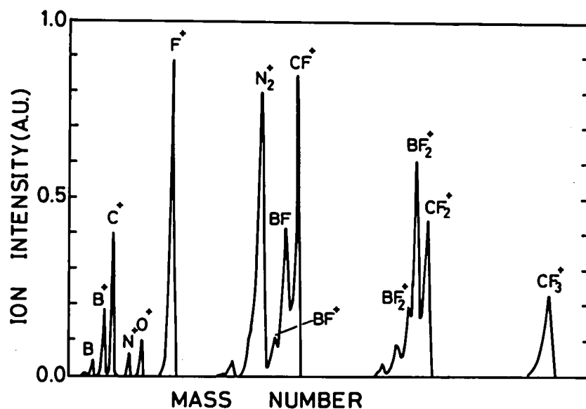
Fig. 4.1 Typical mass spectrum for an ion beam generated by CF_4 gas discharge. The ion extraction voltage is 10 kV and the final kinetic energy of the decelerated ion beam is 1 keV.
