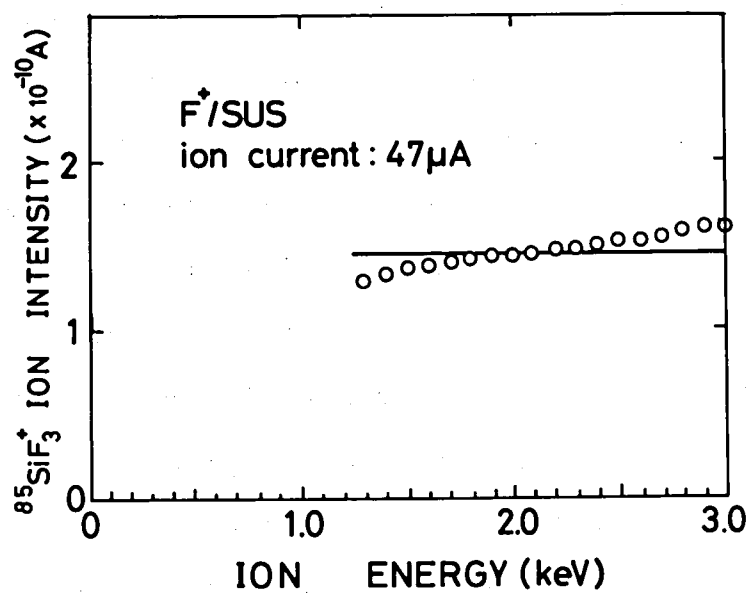
Fig. 4.4 Energy dependence of m/e=85 ion intensity for \text{F}^+/\text{SUS} ion bombardment.
