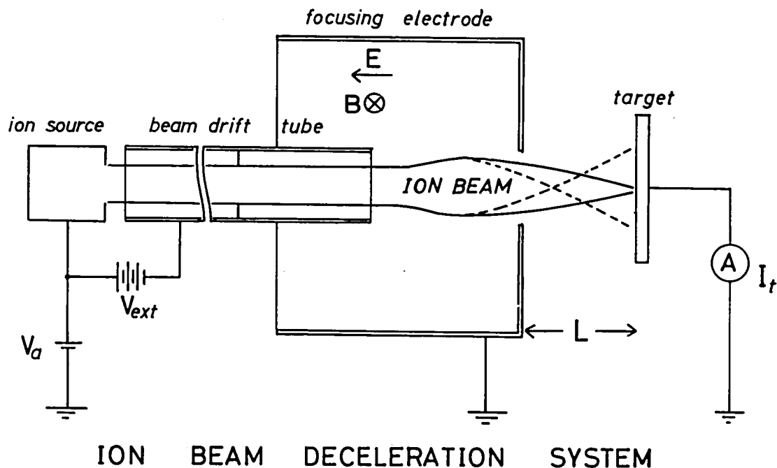
Fig. 2.22 Schematic of an E \times B type ion beam deceleration lens system.
