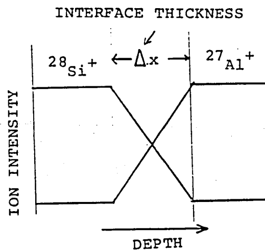
Fig. 3.6 Definition of "interface thickness"
