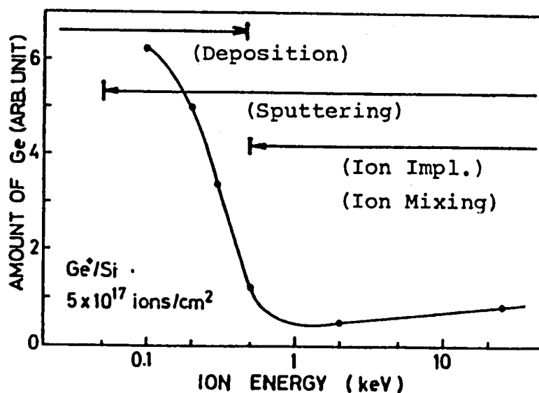
Fig. 3.2 Amount of germanium, measured by XMA, on the surface of a substrate as a function of Ge + ion energy at a constant dose of 5 \times 10^{17} ions/cm 2 .
