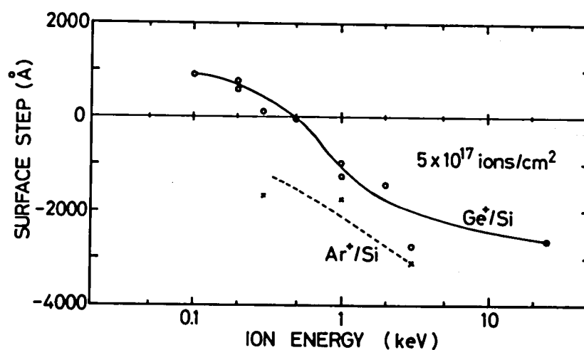
Fig. 3.1 Deposited film thickness or etched substrate depth as a function of incident ion energy. The substrate is a (111) oriented single silicon crystal. Incident ion species are Ge + and Ar + at doses of 5 \times 10^{17} ions/cm 2 .
