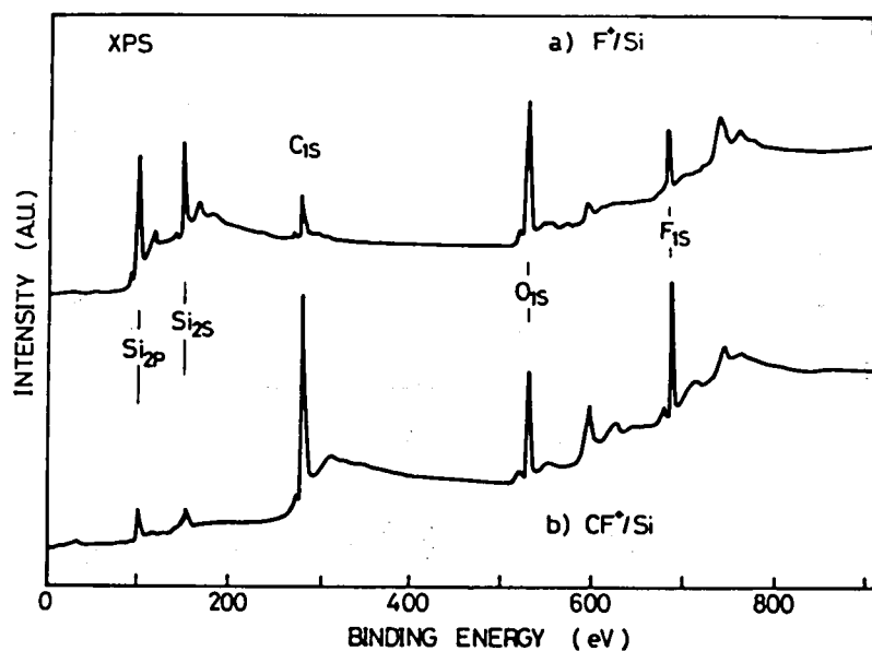
Fig. 4.10 XPS spectra for a silicon surface bombarded by (a) F + and (b) CF + ions. The kinetic energy of the ion beam is 3 keV.
