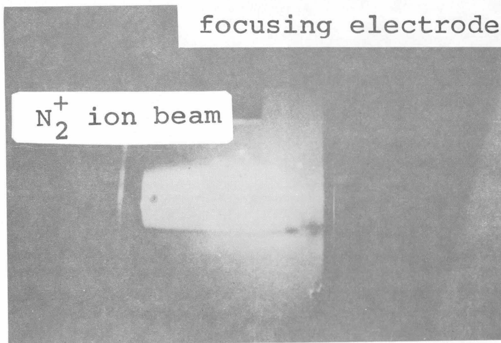
Fig. 2.25 Shape of an N_2^+ ion beam in the case of reflection inside the focusing electrode. eV_{\text{ext}} = 25 \text{ keV} , V_a = -1 \text{ kV} .
