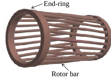
Fig. 1. Schematic diagram of rotor (secondary) windings. Rotor bars are located in the rotor core (silicon steel), and then short-circuited by the end rings [1-6].
