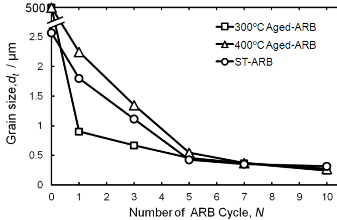
Fig. 3.4. Change in grain size as a function of the number of ARB cycle.
