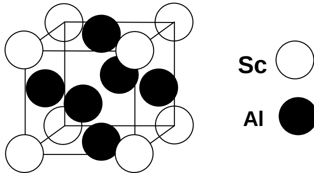
Fig. 1.4. Atomic arrangement of \text{Al}_3\text{Sc} phase [11].
