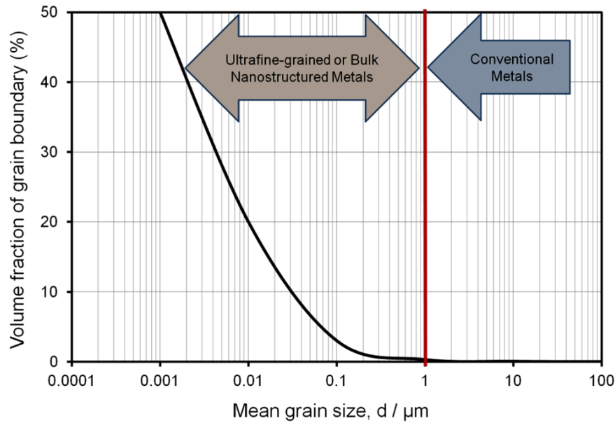
Fig. 1.5. The volume fraction of grain boundary as a function of mean grain size [36].
