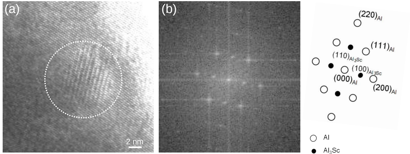
Fig. 2.13. A high-resolution TEM image of a \text{Al}_3\text{Sc} precipitate in the 400°C Aged-ARB specimen deformed by ARB up to 9-cycle. (a) A precipitate having the same orientation relationship with matrix, and (b) corresponding FFT pattern for the area surrounded by broken circular lines in (a).
