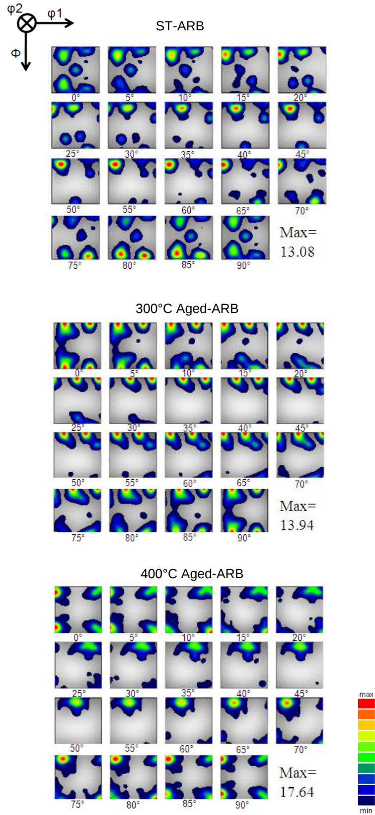
Fig. 5.6. ODF sections of constant \phi_2 showing the texture components in the ST-ARB, 300°C Aged-ARB and 400°C Aged-ARB specimens after annealing at 600°C.
