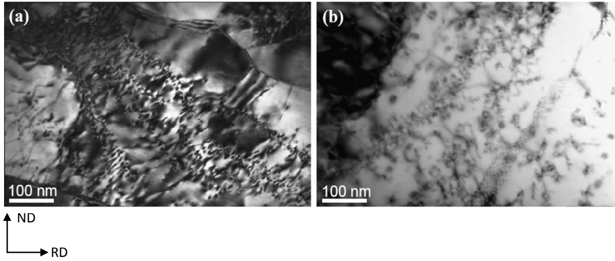
Fig. 2.8. TEM micrographs of the (a) 300°C Aged-ARB 1-cycle and (b) 400°C Aged-ARB 1-cycle specimens.
