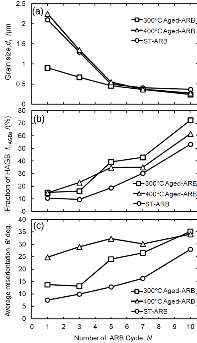
Fig. 2.6. Change in the average grain size, d_b , (a), fraction of high angle boundary, f_{\text{HAGBs}} , (b) and average misorientation, \theta , (c) in the ARB processed specimens as a function of the number of ARB cycles.
