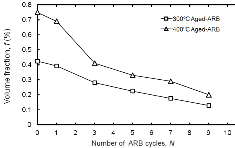
Fig. 3.10. Change in volume fraction of \text{Al}_3\text{Sc} precipitates in the 300°C Aged-ARB specimen and 400°C Aged-ARB specimen as a function of ARB cycle.
