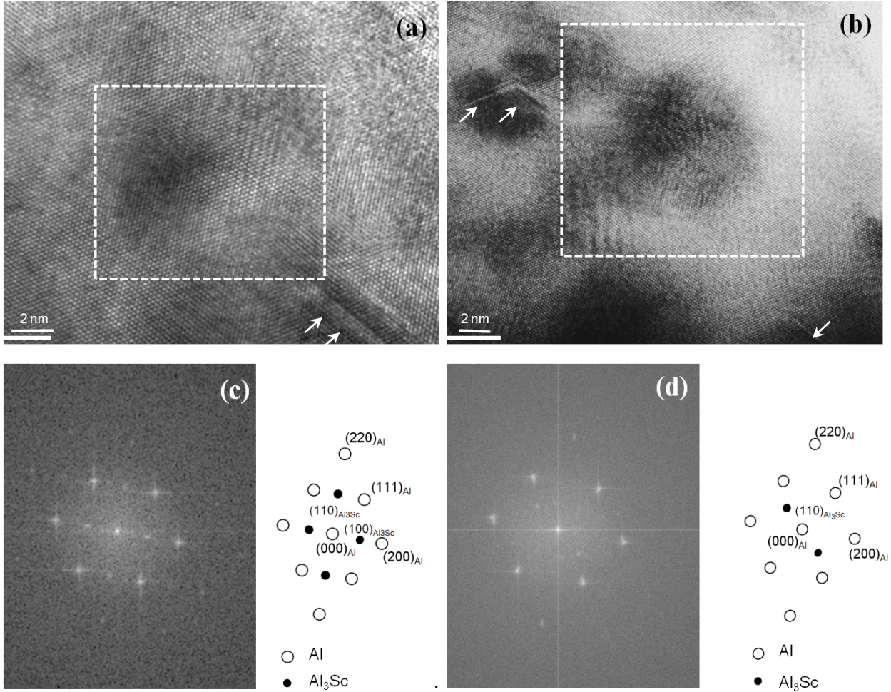
Fig. 2.11. High resolution TEM micrograph of Al 3 Sc precipitates in the 300°C Aged-ARB specimen after 9-cycle of ARB. (a) A precipitate having the identical orientation relationship with matrix, and (b) a precipitate with different orientation relationship with matrix. (c) and (d) are corresponding diffraction patterns obtained by FFT analysis for the areas surrounded by broken lines in (a) and (b), respectively.
