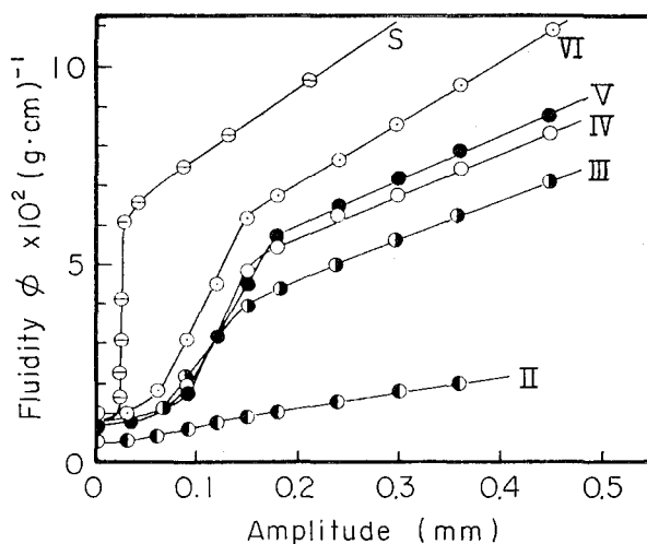
Fig. 7. Relation between the amplitude and the fluidity of powder beds.
