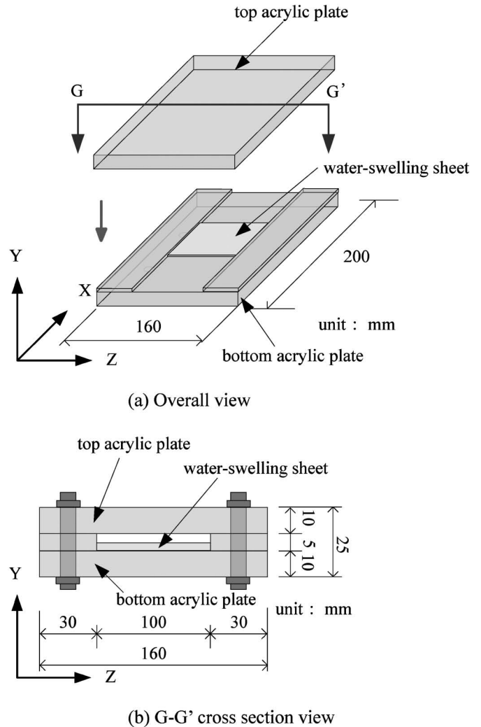
Fig. 23. Specimen for water swelling rate test
