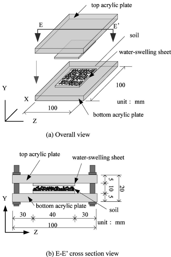
Fig. 19. Specimen for visual check of contact surface after swelling test
