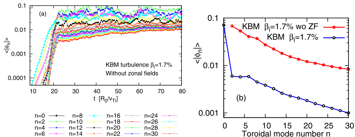
FIG. 12. Time evolution of electrostatic potential for each toroidal mode number without the zonal mode ( n=0 mode) (a) and the toroidal mode number spectrum of the electrostatic potential with and without the zonal mode (b) for KBM turbulence at \beta_i = 1.7\% .
