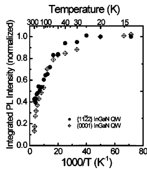
FIG. 3. Temperature dependence of integrated PL intensities of the \{112\bar{2}\} QW and the conventional C -oriented \text{In}_x\text{Ga}_{1-x}\text{N} QW. The intensities were normalized by those at 13 K.
