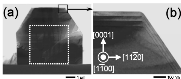
FIG. 1. Cross-sectional STEM images viewed from [1100] direction. (a) Entire region and (b) magnified image of the (0001) and \{1122\} facets. The white broken square indicates the shape of GaN before regrowth.
