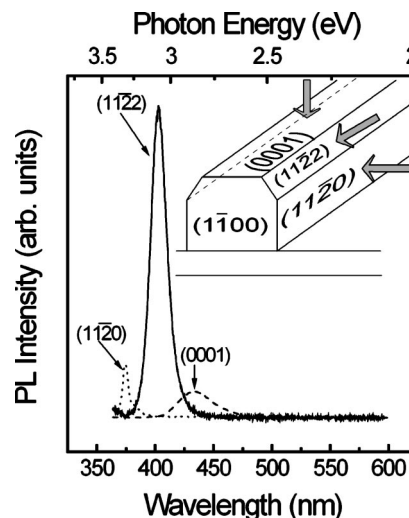
FIG. 2. Microscopic PL spectra from the (1120) , (1122) , and (0001) MQWs at RT. The inset figure shows the schematic sample structure, and arrows indicate the directions for excitation and collection.
