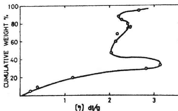
Fig. 12 Cumulative weight distribution curve obtained from polymer particles having an average diameter of 100\mu (polymer load 5.0 g). The polymer particles were packed in the fractionation column by the method shown in Figure 4.
