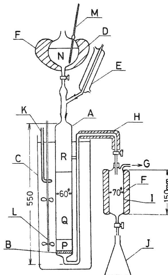
Fig. 1 Fractionation apparatus for the R.T. method.
