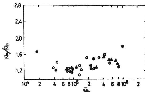
Fig. 8 D values of the fractions: (●) the fractions obtained from the polymer deposited in the 100 % decalin system; (○) in the 70 % decalin system; and (Δ) in the reversed desposition.
