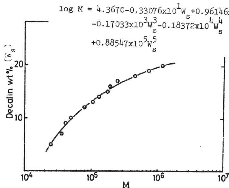
Fig. 8 Relation between the molecular weight and solvent concentration of the cloud point in decalin-butyl carbitol system at the temperature 161°C.
