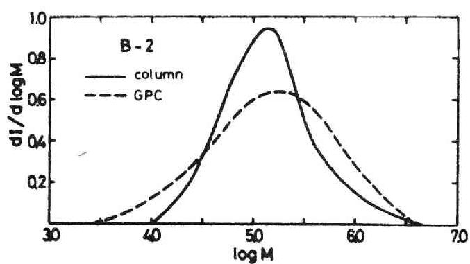
Fig. 14 Molecular weight distribution curves obtained by column fractionation (—) and GPC (-----). Sample B-2.
