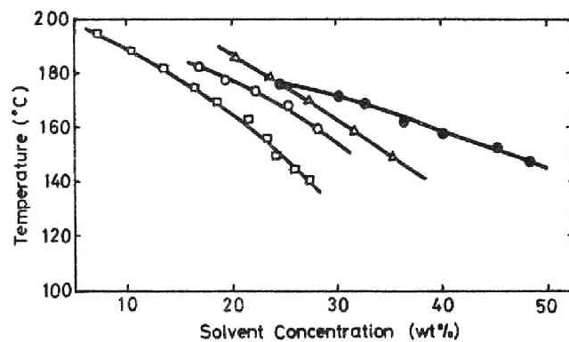
Fig. 2 Cloud points of crystalline polypropylene in solvent-nonsolvent (butyl carbitol) systems. \square : n-hexadecane, \circ : chlorobenzene \Delta : o-dichlorobenzene, \bullet : \alpha -chloronaphthalene Polymer concentration : 1.0 wt% polymer/(solvent + nonsolvent).
