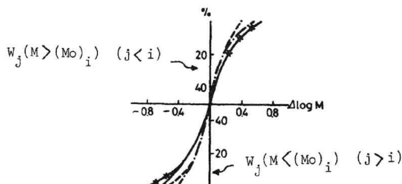
Fig. 15 Distribution curves of the fractions from sample C-1: (-----) fractions 5-9, (- - -) fractions 2-4 and 10-13, (——) fractions 14-16, (-x-x-) fraction 1. \Delta \log M = (\log Mo)_i - (\log Mo)_j , (\log Mo)_i is the peak position of distribution curve of i-th fraction, and (\log Mo)_j is that of j-th fraction.
