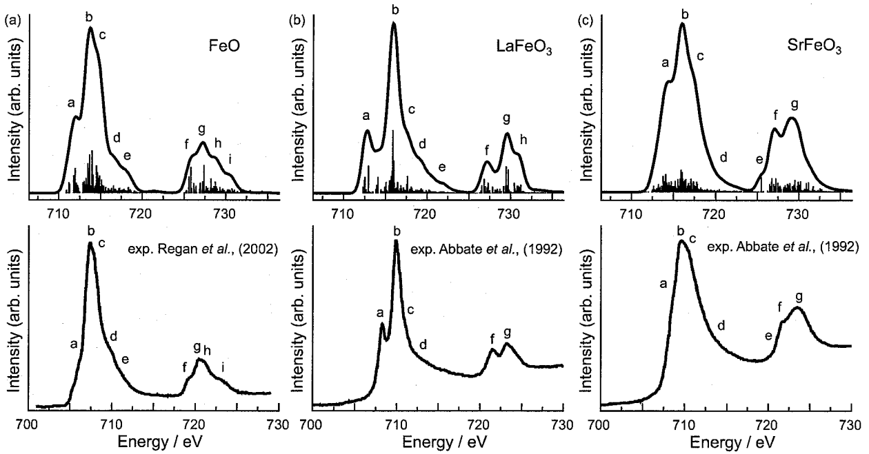
Figure 3.2: Theoretical Fe L_{2,3} -edge NEXAFS in (a) FeO, (b) \text{LaFeO}_3 and (c) \text{SrFeO}_3 (upper panel), and corresponding experimental NEXAFS spectra. Bars in the upper panel show oscillator strength with many-electron eigenvalues before the Gaussian broadening. Experimental NEXAFS spectra are adapted with permission from Refs. [10] and [11]. Copyrighted (2006) American Physical Society.
