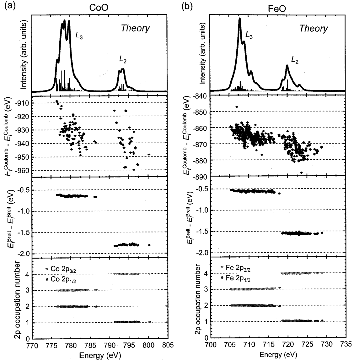
Figure 6.5: (upper) TM L_{2,3} -edge NEXAFS of (a) CoO and (b) FeO. (2nd upper) Difference of Coulomb interaction energy between initial and final states of TM L_{2,3} -edge NEXAFS ( E_f^{\text{Coulomb}} - E_i^{\text{Coulomb}} ). (2nd lower) Difference of Breit interaction energy between initial and final states of TM L_{2,3} -edge NEXAFS ( E_f^{\text{Breit}} - E_i^{\text{Breit}} ). (lower) Expectation values of occupation number of TM- 2p_{1/2} and TM- 2p_{3/2} orbitals at the final states of TM L_{2,3} -edge NEXAFS.
