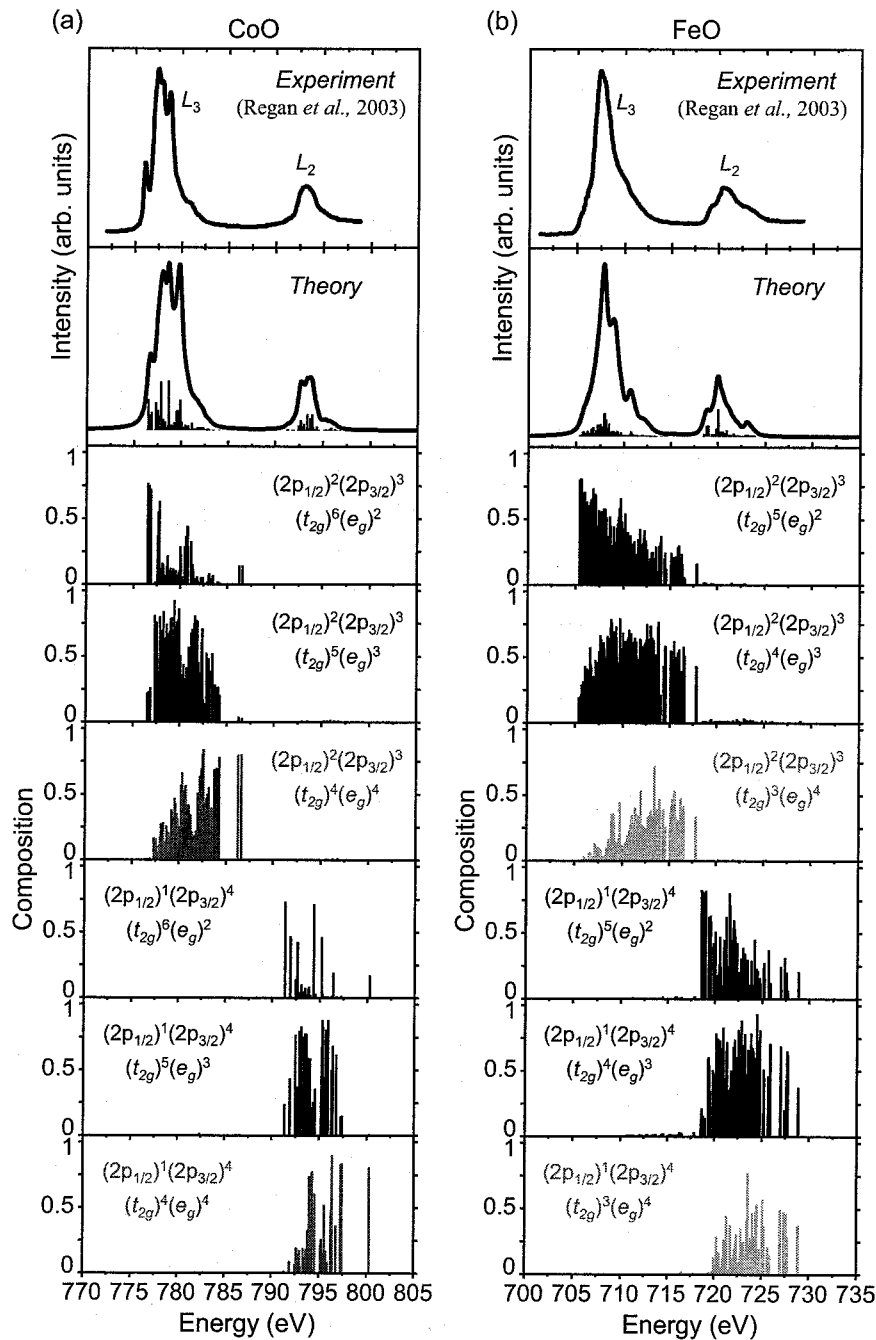
Figure 6.1: Theoretical TM L_{2,3} -edge NEXAFS of (a) CoO and (b) FeO compared with experimental spectra adapted with permission from Ref. [19] (Copyrighted (2006) American Physical Society). Solid bars in the upper panel show the oscillator strengths for the many-electron eigenstates. The following panels show the composition of final configurations for the many-electron eigenstates. The transitions to the final configurations drawn in light gray lines have little contribution to the oscillator strength of L_{2,3} -edge NEXAFS.
