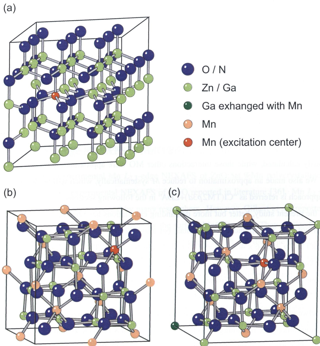
Figure 5.1: Atomic arrangement of (a) (\text{Zn}_{31}\text{MnO}_{32}) / (\text{Ga}_{31}\text{MnN}_{32}) supercell, (b) \text{Mn}_8\text{Ga}_{16}\text{O}_{32} unit cell of \text{MnGa}_2\text{O}_4 normal spinel and (c) (\text{Mn}_7\text{Ga})(\text{Ga}_{15}\text{Mn})\text{O}_{32} unit cell where one of Mn (red ball) was exchanged with a furthest Ga atom (dark green ball). Cluster models composed of excitation center Mn (red ball) and nearest-neighbor O / N atoms were constructed after geometry optimization.
