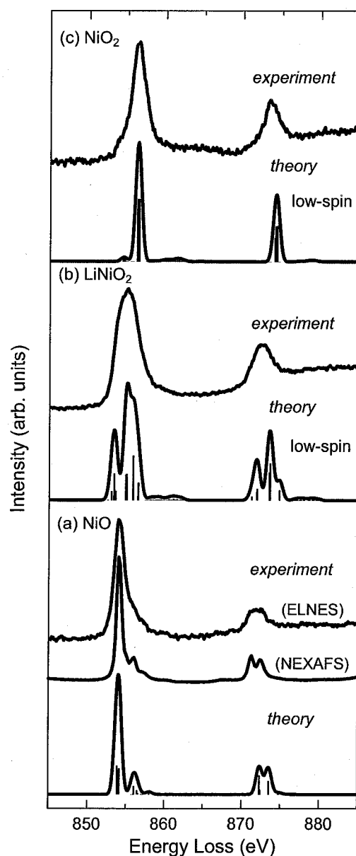
Figure 4.5: Experimental Ni L_{2,3} -edge ELNES of (a) \text{NiO} , (b) \text{LiNiO}_2 , and (c) \text{NiO}_2 as compared to theoretical spectra. For \text{NiO} , Ni L_{2,3} NEXAFS with a higher energy resolution is also shown to see detailed structures. For theoretical spectra of \text{LiNiO}_2 and \text{NiO}_2 , low-spin states are chosen as initial states. The absolute transition energy of the theoretical spectrum of \text{NiO} , \text{LiNiO}_2 , and \text{NiO}_2 are shifted by 1.9, 1.6, and 1.2 eV, respectively, in order to see best matches with experimental spectra.
