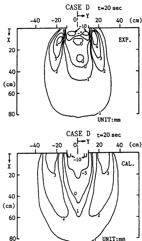
Fig. 13. Comparison between the calculated results of bed level distribution and the experimental ones in CASE D.
