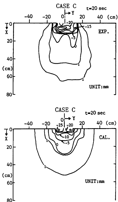
Fig. 12. Comparison between the calculated results of bed level distribution and the experimental ones in CASE C.
