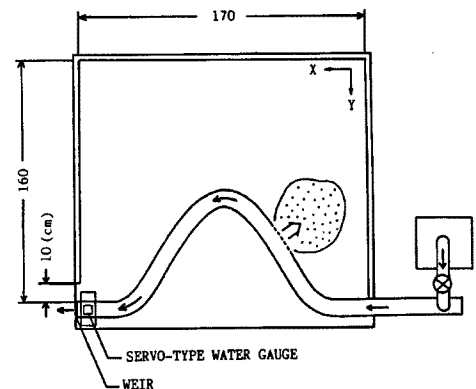
Fig. 17. Experimental set-up for two-dimensional suspended sediment deposition.
