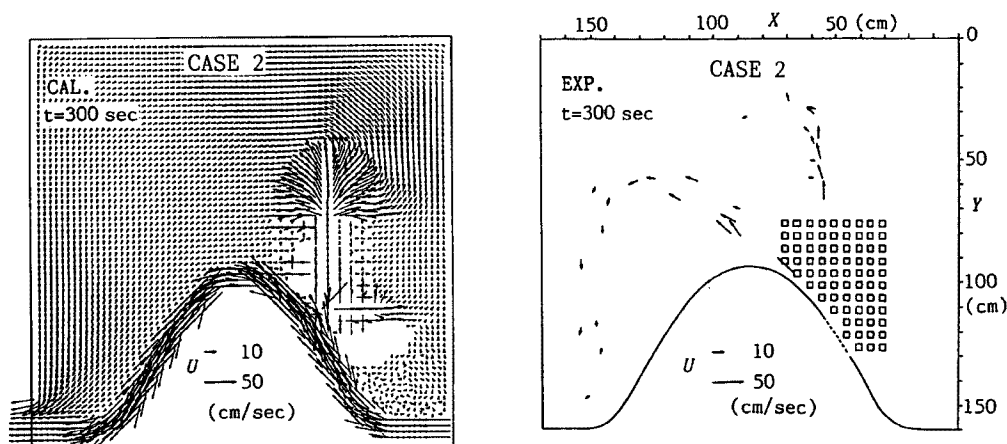
Fig. 24. Velocity distributions both in the calculation and the experiment (CASE 2).
