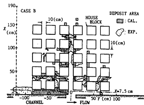
Fig. 10. Comparison between the calculated deposition area and the experimental one in CASE B.
