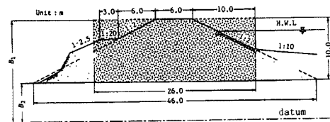
Fig. 27. Standard cross section of embankment used for the Kizu river at 6~31 km upstream from confluent of three rivers, the Kizu, the Uji and the Katsura river.
