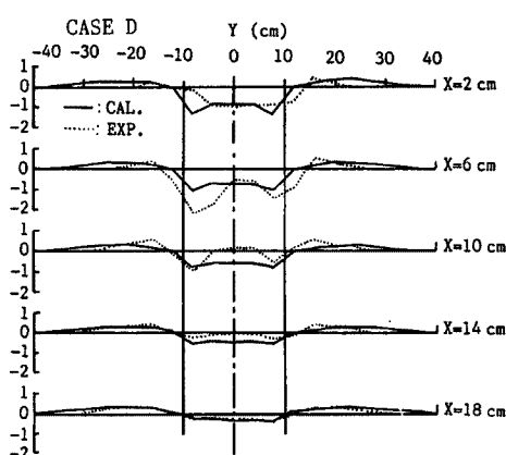
Fig. 15. Comparison between the calculated cross sectional bed configurations and the experimental ones in CASE D.
