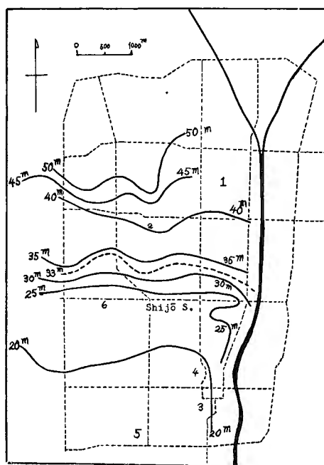
Fig. 2 Contour lines of ground water levels in Kyoto City, Aug. 1962.
