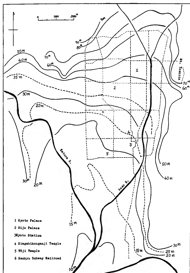
Fig. 1 Contour lines of ground water levels in Kyoto City, Jan. 1958. (Numbers attached to Curves are heights in m T.P.)
