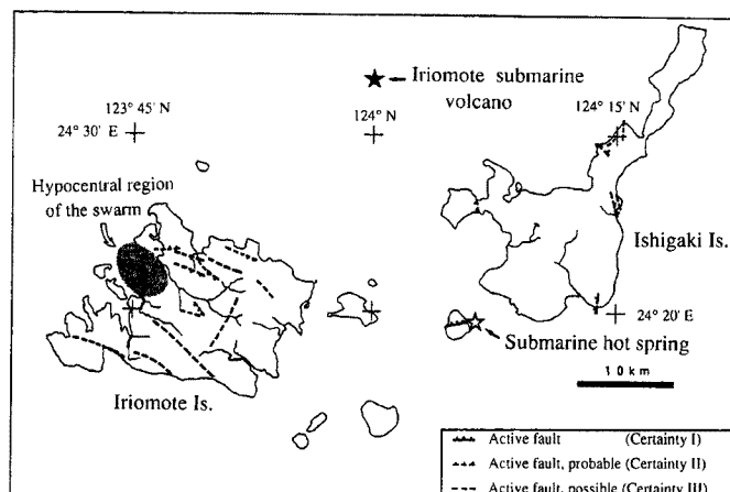
Fig. 11. Distribution of active faults on Iriomote island 12,9,16) .
