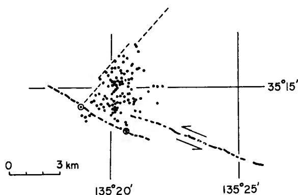
Fig. 7. Detailed traces of the Mitoke Fault with the epicentral distribution of the aftershocks. The dotted line is the same as those shown in Fig. 5.
