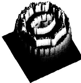
Figure 5: The graph of z \mapsto [(\partial T_{\infty, \tau_a}(z)/\partial a_1)]|_{a_1=1/2} , where, \tau_a is the element in Figure 3. A complex analogue of the Takagi function.
