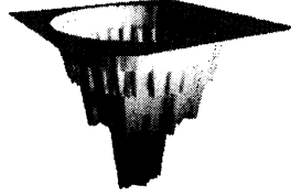
Figure 3: The graph of z \mapsto T_{\infty, \tau_{1/2}}(z) , where, letting (h_1, h_2) be the element in Figure 2, we set \tau_a := \sum_{j=1}^2 a_j \delta_{h_j} . A devil's coliseum (a complex analogue of the devil's staircase). \tau_a is mean stable. The set of varying points is equal to Figure 2.
