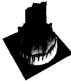
Figure 4: The graph of z \mapsto T_{0, \tau_{1/2}}(z) , where, letting (h_1, h_2) be the element in Figure 2, we set \tau_a := \sum_{j=1}^2 a_j \delta_{h_j} . Figure 3 upside down. A “fractal wedding cake”.
