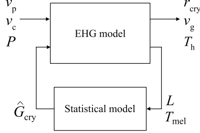
Fig. 7: Structure of the gray-EHG model.
