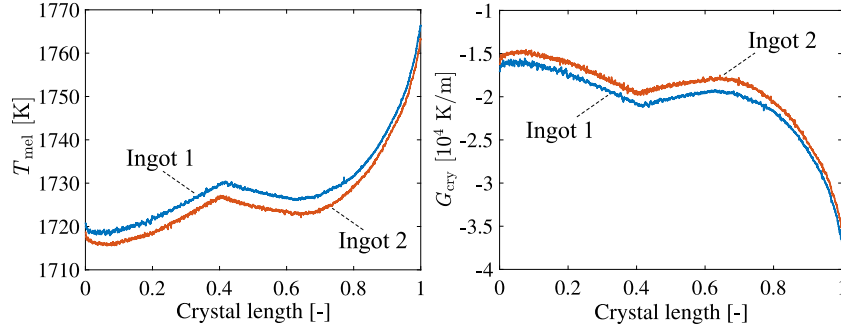
Fig. 8: Calculated melt temperature T_{\text{mel}} and temperature gradient in the crystal at the solid-liquid interface G_{\text{cry}} using the real process data of the ingots 1 and 2.
