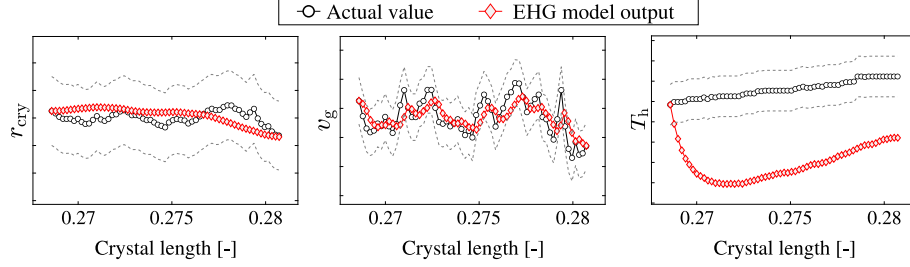
Fig. 6: Prediction result of the crystal radius r_{\text{cry}} , the crystal growth rate v_g , and the heater temperature T_h by the EHG model. The horizontal axis is the dimensionless crystal length. To protect confidentiality the scales of the vertical axis are shown in an arbitrary unit. The range between the dotted lines represents the tolerance of the prediction error.
