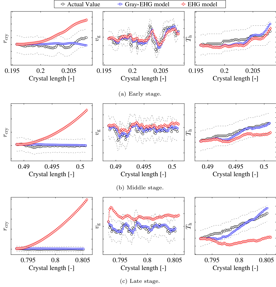
Fig. 12: Prediction results of the crystal radius r_{\text{cry}} , the crystal growth rate v_g , and the heater temperature T_h at three stages in data of the ingot 3. To protect confidentiality the scales of the vertical axis are shown in an arbitrary unit. The range between the dotted lines shows an acceptable error.
