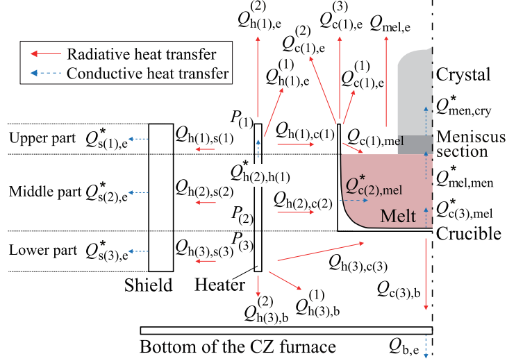
Fig. 3: Heat transfer calculated in the energy transfer model.
