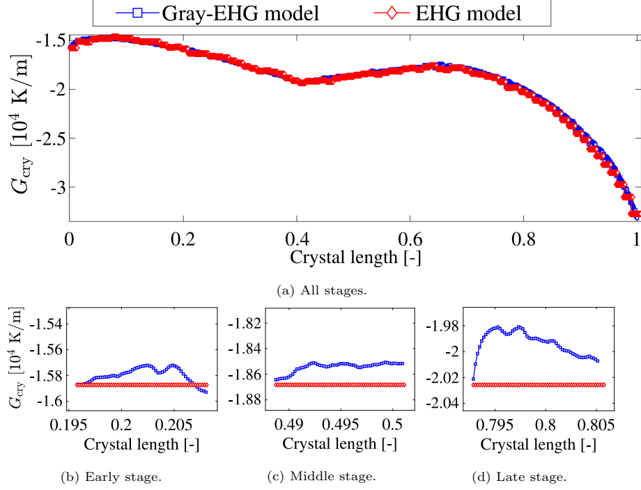
Fig. 13: Temperature gradient in the crystal at the solid-liquid interface G_{\text{cry}} used for prediction in the data of the ingot 3 by the EHG model and the gray-EHG model.
