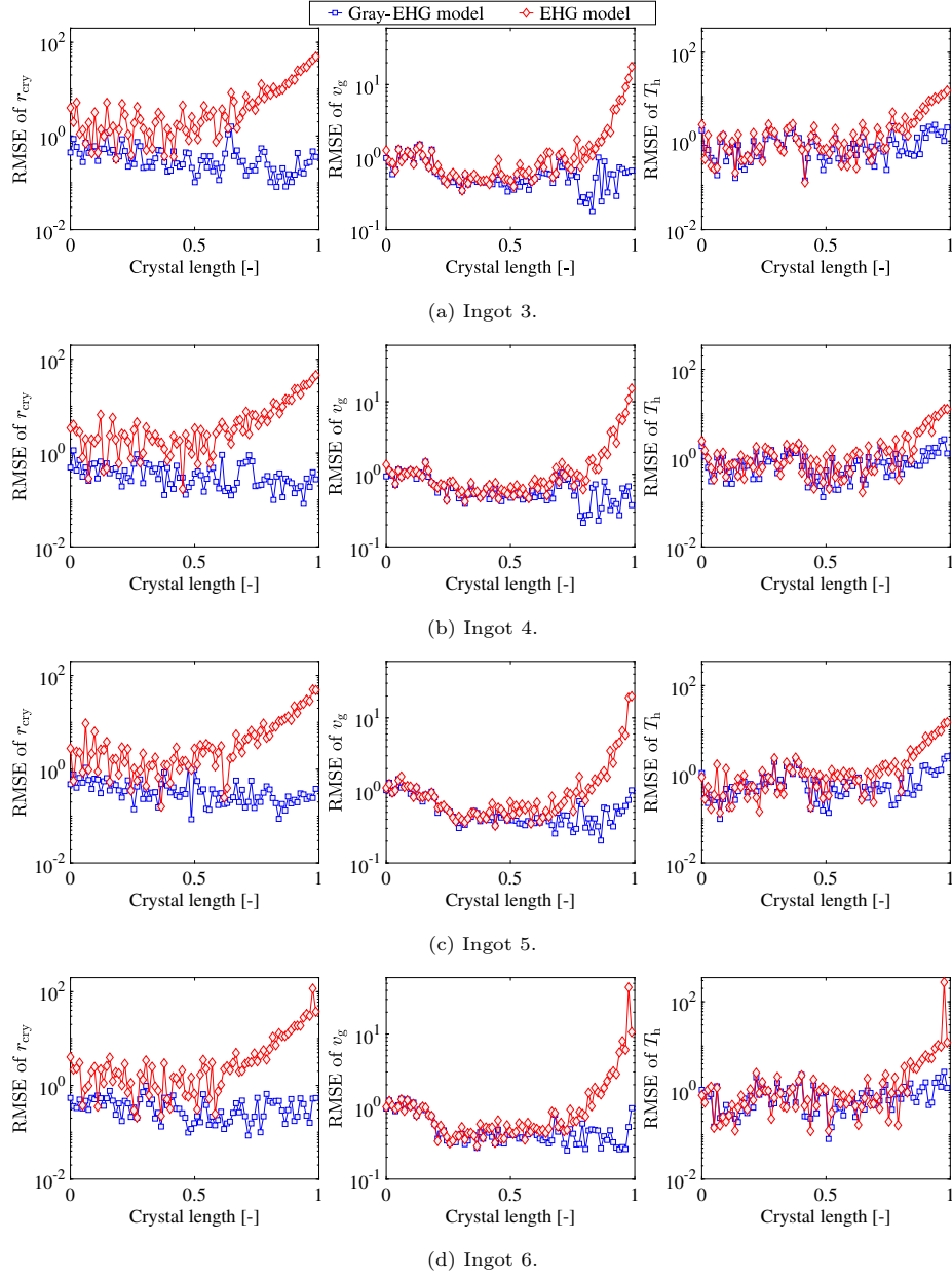
Fig. 11: RMSEs of the crystal radius r_{\text{cry}} , the crystal growth rate v_g , and the heater temperature T_h against the data of the ingots 3 to 6. The horizontal axis is the dimensionless crystal length.
