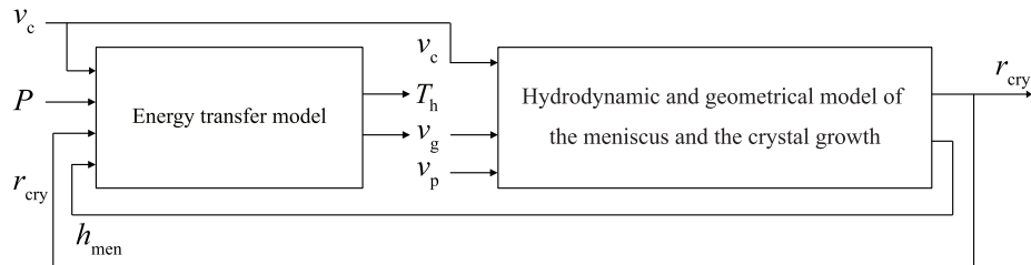
Fig. 2: Structure of the EHG model.
