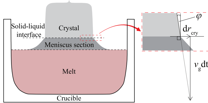
Fig. 5: Geometrical relationship around the solid-liquid interface.
