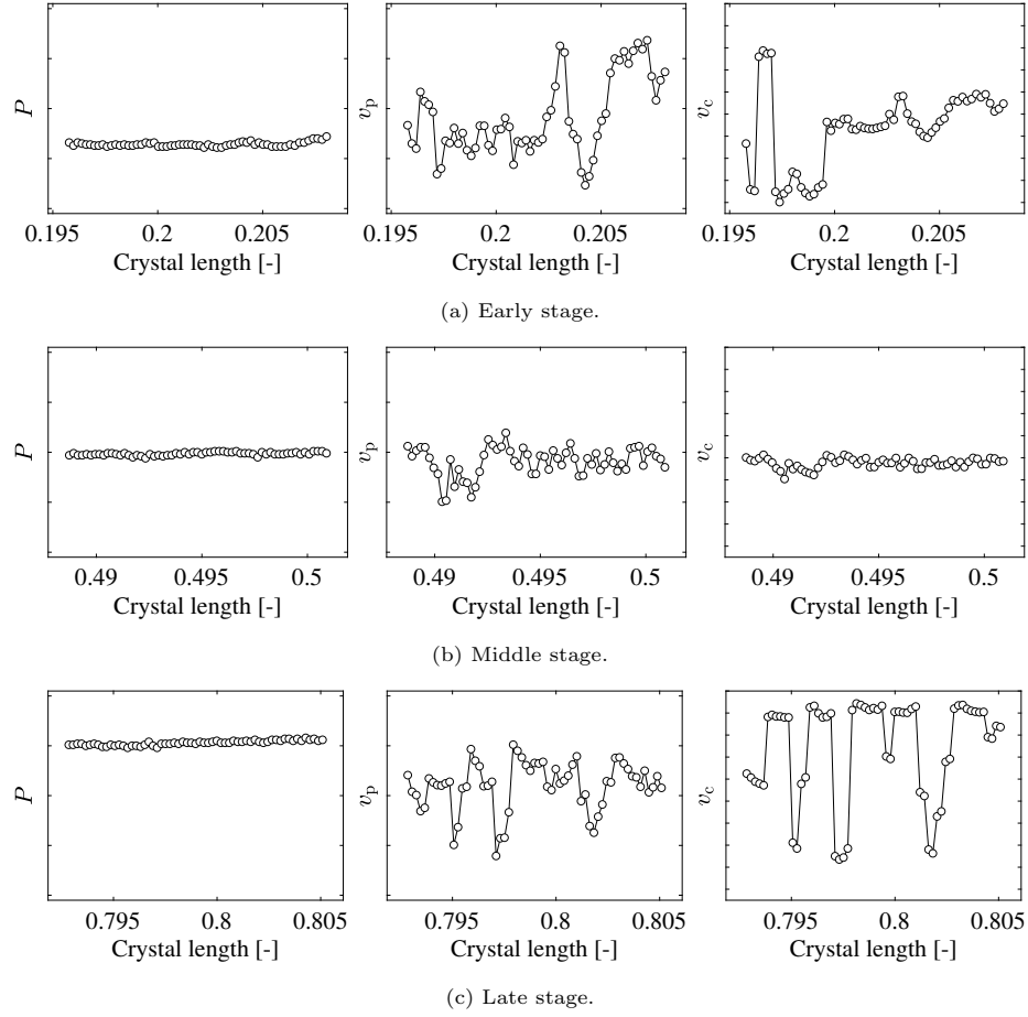
Fig. 10: Input variables at three stages in data of the ingot 3. The values of the vertical axis are not shown to protect confidentiality.
