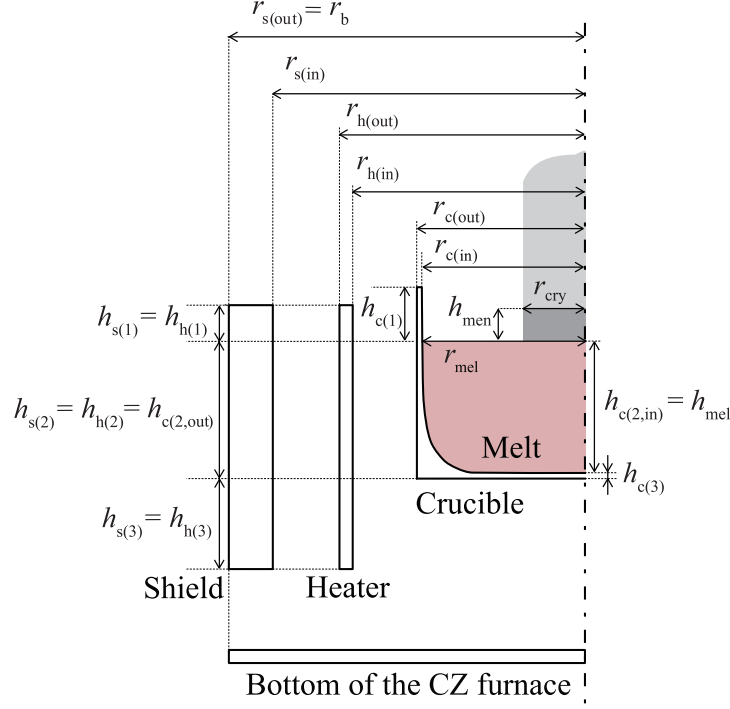
Fig. 4: Definition of the radius and the height of each component of the Czochochalski process.
