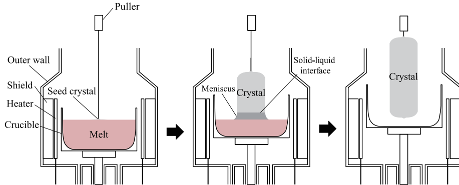
Fig. 1: Schematic diagram of the CZ process.
