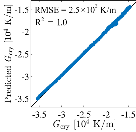
Fig. 9: Temperature gradient in the crystal at the solid-liquid interface G_{\text{cry}} predicted by the statistical model using the data of ingot 2.
