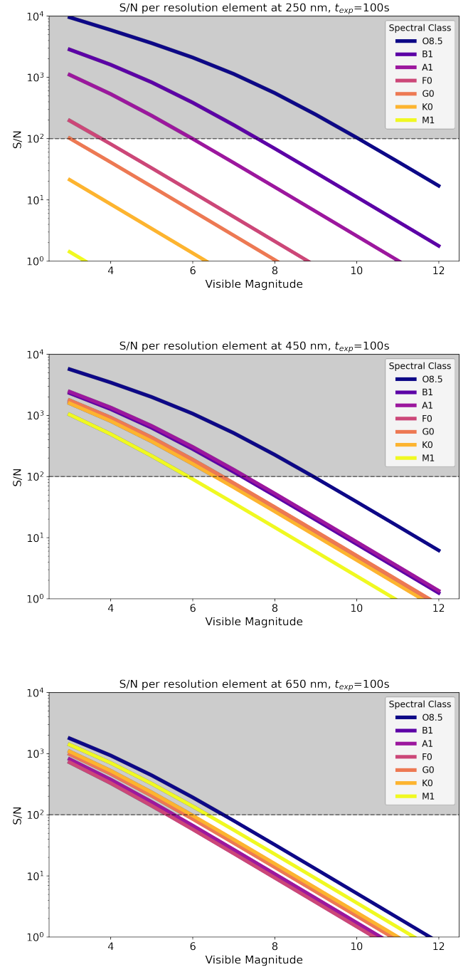
Figure 1. Expected Mauve S/N per resolution element (10.5 nm) at 250 nm, 450 nm and 650 nm for a 100 s exposure time for different stellar types. The performance at the faint end is likely to be limited by the capacity of the spacecraft to track the target, which depends on factors such as stellar type and the presence of other sources in the field. Performance may also be constrained by systematics (e.g., noise saturation) at S/N per resolution element higher than 100. This is indicated in the plots as a shaded grey region above the dashed line.
