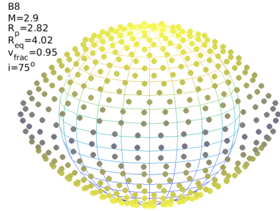
Figure 7. The distorted surface of a B8V star (mass 2.9 M_{\odot} , polar radius 2.82 R_{\odot} ) rotating at 95% of its critical velocity (363 km/s) seen at an inclination angle i = 75^{\circ} ( i = 0^{\circ} corresponds to a star viewed pole-on). The coloured circles represent surface “patches” that can be seen by a distant observer. Gravitational darkening is illustrated by the colour of each patch, ranging from bright yellow for the hot pole ( T_{\text{eff}} = 13,000 K) to dark grey for the cooler equator ( T_{\text{eff}} = 8000 K). To compute the SED seen by a distant observer, the intensity for each surface patch is computed using local values of ( T_{\text{eff}} , \log g ), and then intensities for all patches are summed, weighted by their solid angles.
