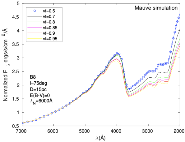
Figure 9. Predicted SEDs for the star of Figure 7 as a function of the stellar rotation rate v_{\text{frac}} (see legend). The SEDs have been convolved to the same resolution as Mauve ( R = 50 ) and are normalised to unity at \lambda = 6000 \text{ \AA} .
