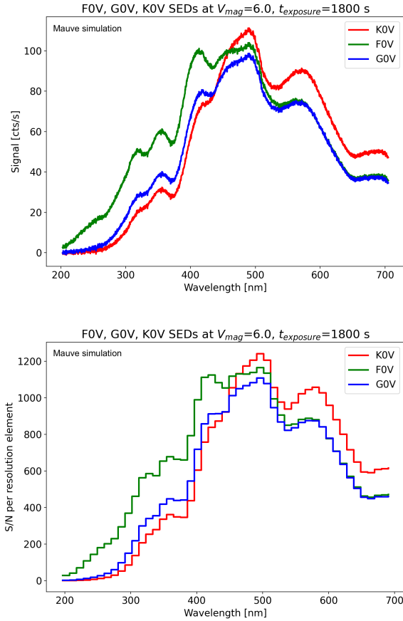
Figure 6. Simulated Mauve SEDs (upper panel) and S/N (lower panel) for example K0V, G0V and F0V stars at V_{\text{mag}} = 6 using an exposure time of 30 minutes.
