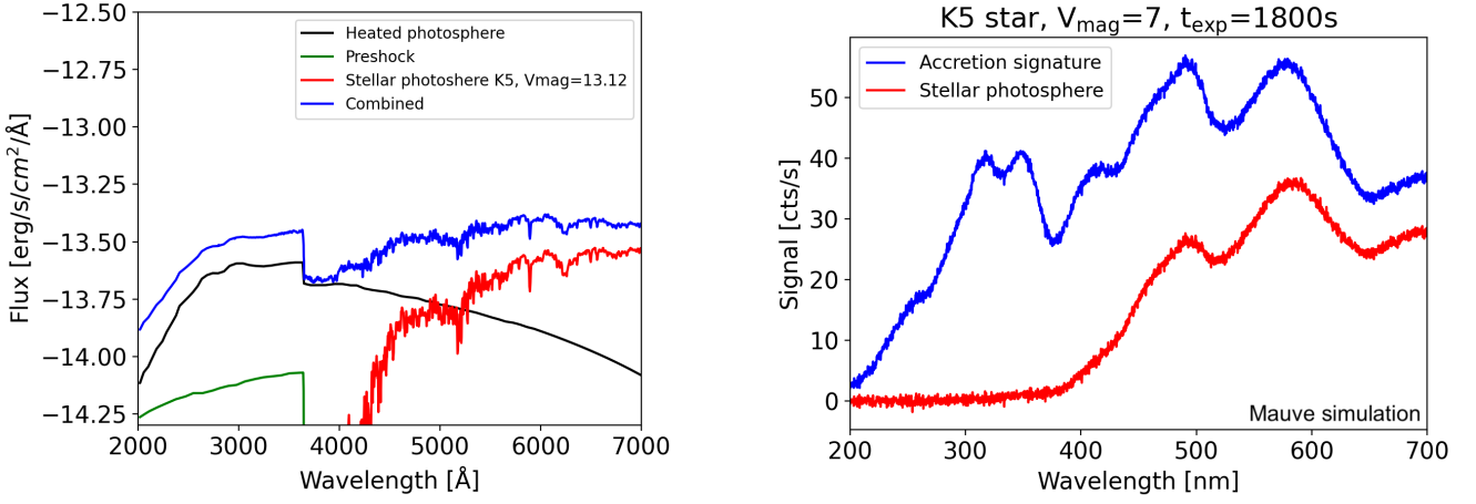
Figure 16. Left: SED of a pre-main sequence star at V_{\text{mag}}=13.12 displaying accretion (blue line) which includes contributions from the preshock (green line), heated photosphere–postshock (black line) and stellar photosphere (red line). Figure reproduced from Hartmann et al. (2016) . Right: Mauve simulated data for the accreting model versus the non-accreting (quiet) photosphere for a brighter K5 star.
