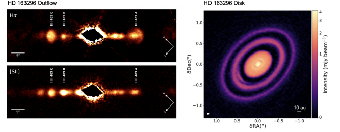
Figure 14. Left: VLT/MUSE observations of the bipolar jet driven by the Herbig Ae/Be star HD 163296 taken from Kirwan et al. (2022). Right: Map of the HD 163296 disk recorded in the 1.25 mm continuum taken from Isella et al. (2018). The dust rings and sub-structures are interpreted as evidence that planet formation processes are active in the disk.
