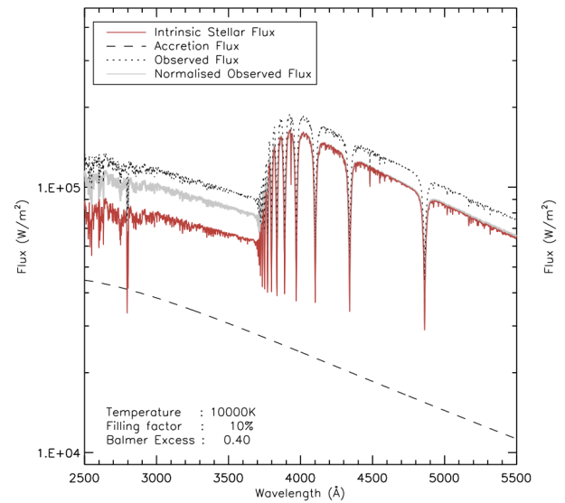
Figure 11. From Fairlamb et al. (2015). The red spectrum is an A0 photosphere and the black dashed line shows the accretion flux. These sum to produce the observed black dotted spectrum, which when renormalised to match the photospheric (red) spectrum longward of the Balmer jump produces the light gray spectrum showing a substantial excess shortward of the Balmer jump.
