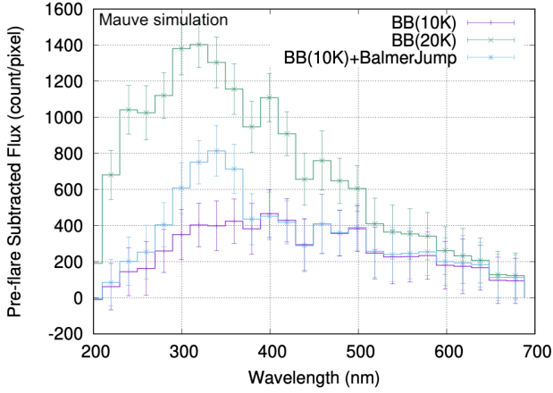
Figure 4. Comparison of simulated spectra based on different models for flare continuum. The flare amplitude for all models is 2.4% in the TESS bandpass. The error bars represent three standard errors of mean for each bin.
