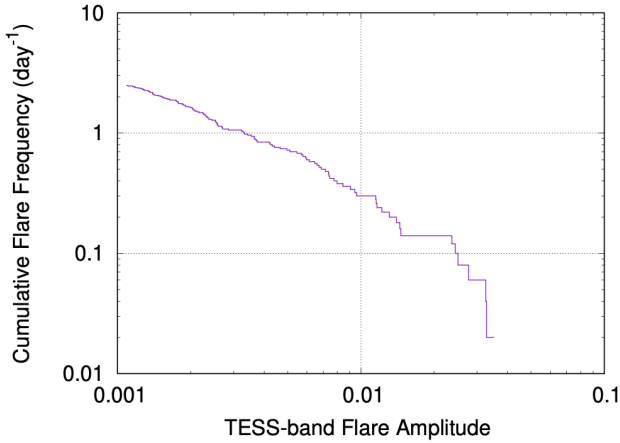
Figure 3. Cumulative flare frequency for AU Mic as a function of the flare amplitude in the TESS bandpass (600–1000 nm). The flare data are taken from Ikuta et al. (2023).
