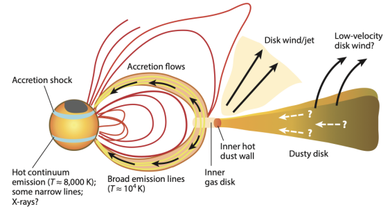
Figure 10. From Hartmann et al. (2016). The close circumstellar environment of a classical T Tauri star. Strong stellar fields truncate the accretion disk near the co-rotation radius, directing accreting material along the field lines where bright accretion shocks form.
