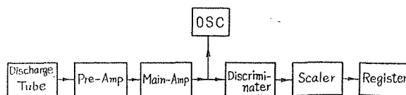
Fig. 2. Block diagram of the apparatus.
