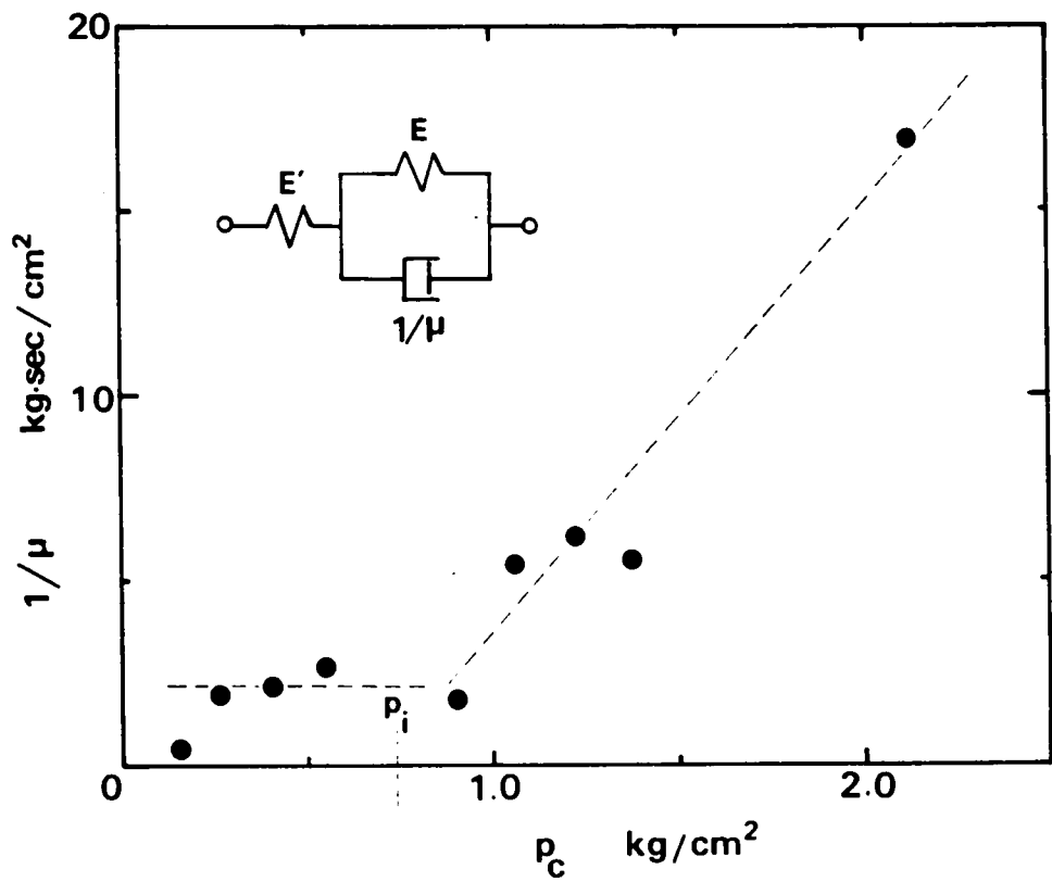
Fig.4.18 Variation of 1/\mu with the confining pressure ( p_i : the pre-consolidation pressure).
