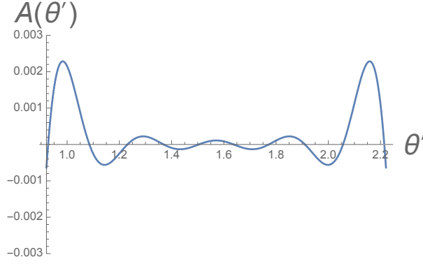
Figure 19: A plot of the amplitude (5.29) for n = 11 , magnified around \theta' = \pi/2 .
