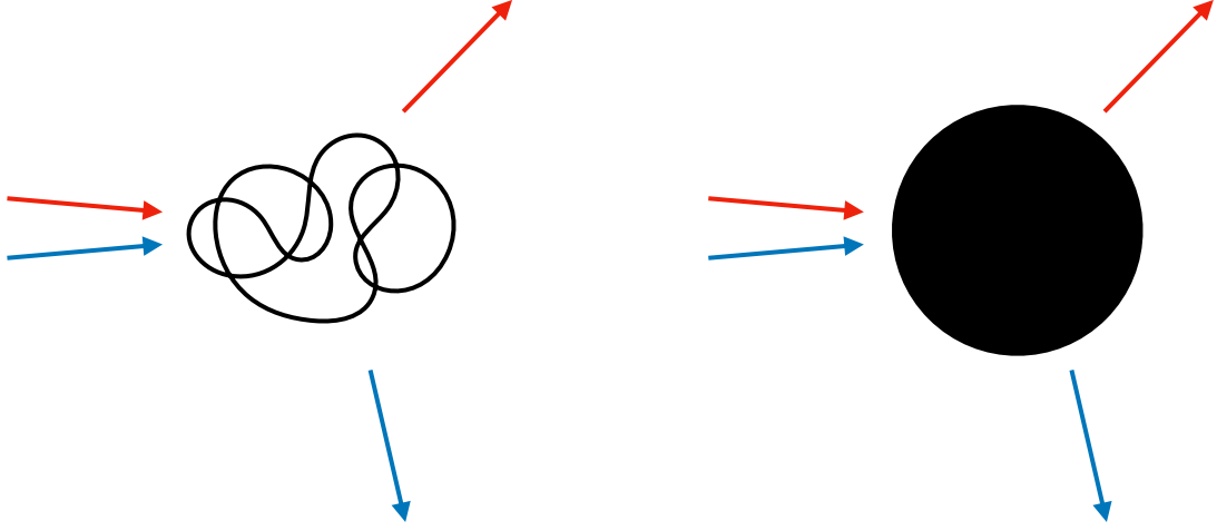
Figure 1: A highly excited string and a black hole are expected to be chaotic scatterers. When a particle is shot into a black hole, its initial conditions are apparently forgotten due to the thermalization, and it takes a long time for a particle to escape due to the redshift near the event horizon. Actually, initial condition sensitivity and a long delay-time are typical features of chaotic scatterers. We look for its microscopic origin in scatterings of a highly excited string.
