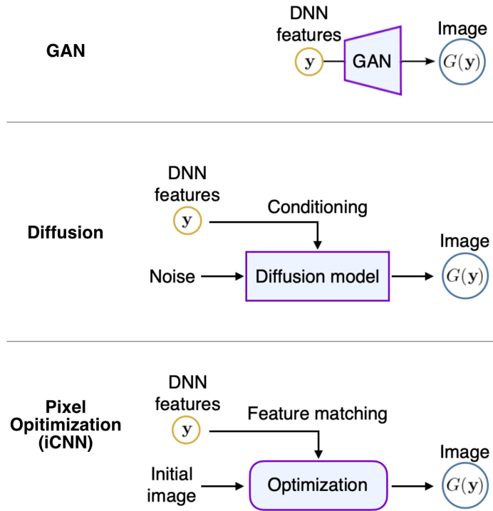
Fig. 6.7 Illustration of image generation with DNN features as the input. Three different generators are shown: Generative Adversarial Network (GAN) generator (top), conditional diffusion model (middle), and pixel optimization (bottom). Both GAN and diffusion models necessitate pre-training on extensive natural image datasets.
