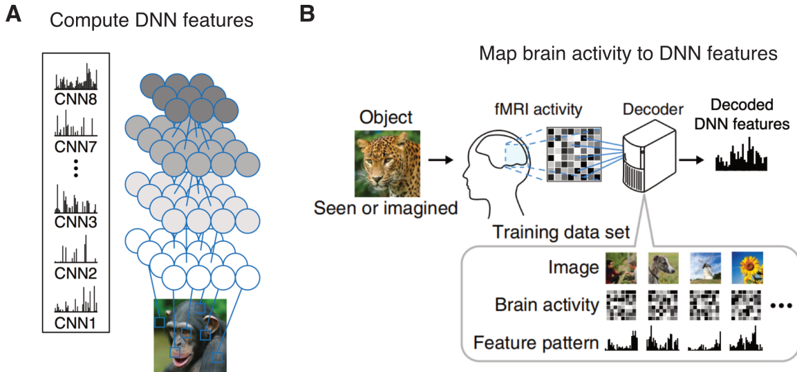
Fig. 3.4 Generic decoding of object category based on DNN representations. Figure adapted from Horikawa and Kamitani (2017).
