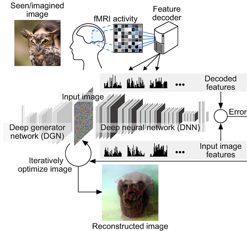
Fig. 3.5 Reconstruction of seen, imagined, or attended images. Figure from Shen et al. (2019a).
