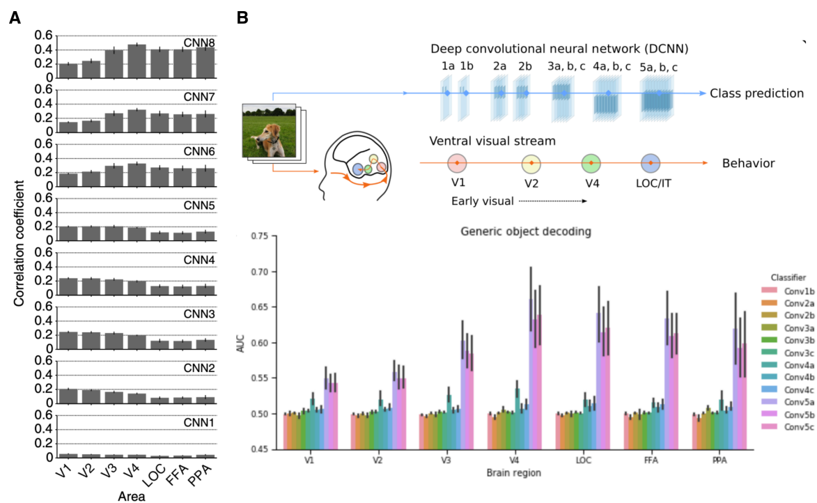
Fig. 3.2 Hierarchical representational correspondence between brain and DNN. While (A) evidence suggests some degree of hierarchical correspondence, (B) the extent and nature of the relationship between brain processing and DNNs remain debated. Figure adapted from Horikawa and Kamitani (2017) and Sexton and Love (2022).
