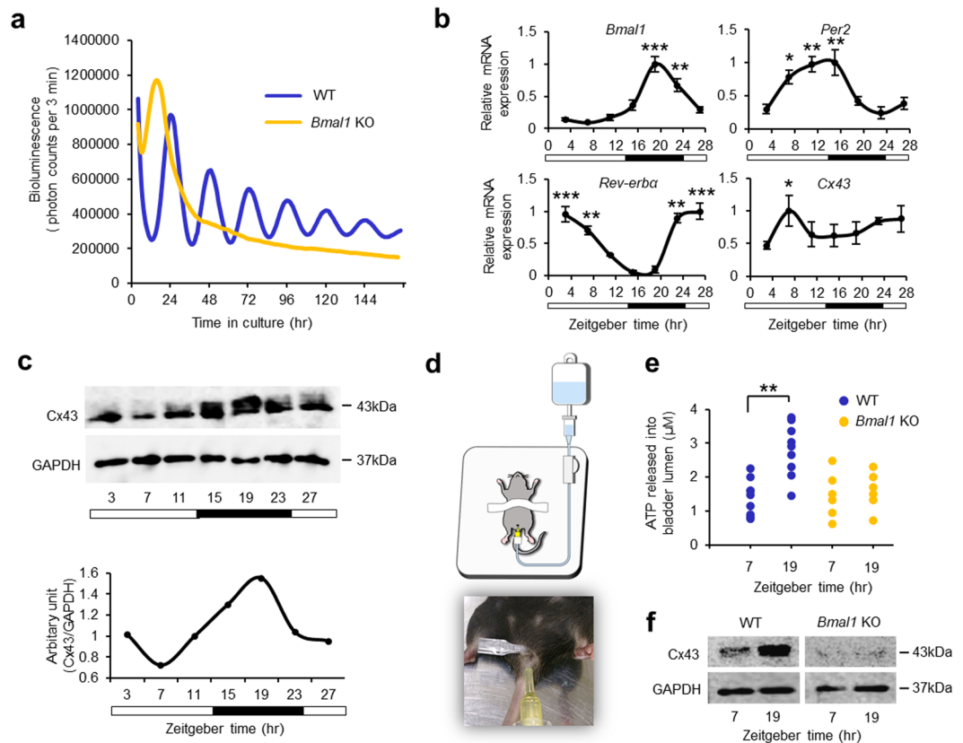
Figure 2. Oscillation of Cx43 and Clock gene expression in mouse urothelium. (a) Representative oscillation of bioluminescence in the urothelium obtained from Per2::luc mice from an ex vivo culture. The period of oscillation was 24.13 \pm 0.07 (mean \pm s.e.m) ( n = 3 ). The oscillation of bioluminescence in Per2::luc/Bmal1 -/- mice were lost completely. (b) Temporal mRNA accumulation of Bmal1 , Per2 , Rev-erba and Cx43 in the urothelium from mice under LD condition. * P < 0.05 , ** P < 0.01 and *** P < 0.001 vs. the nadir value (ZT 7 in Bmal1 , ZT 23 in Per2 , ZT 15 in Rev-erba and ZT 3 in Cx43 ) by one-way ANOVA with Tukey's post hoc test ( n = 4 for each time point). The P -values with Cosinor analysis in Bmal1 , Per2 , Rev-erba and Cx43 were 0.02, 0.002, 0.005 and 0.1 respectively. ZT; Zeitgeber time. (c) Representative temporal Cx43 protein accumulation in the mice urothelium under LD condition as shown by immunoblotting (Cosinor analysis, P = 0.01 ). Full-length blots are presented in Supplementary Fig. S11. (d) A schematic image and photograph of bladder distention to measure the concentration of ATP released into the bladder. (e) Temporal change in the concentration of ATP release after bladder distention. The high/low level was in accord with the Cx43 expression in the urothelium of mice. ** P < 0.01 by Student's t -test ( n = 9 ), which was completely lost in Bmal1 -knockout mice ( n = 6 ). (f) Circadian change of Cx43 protein expression in the urothelium of wild-type mice was lost in Bmal1 -knockout mice. Full-length blots are presented in Supplementary Fig. S11. All error bars indicate s.e.m.
