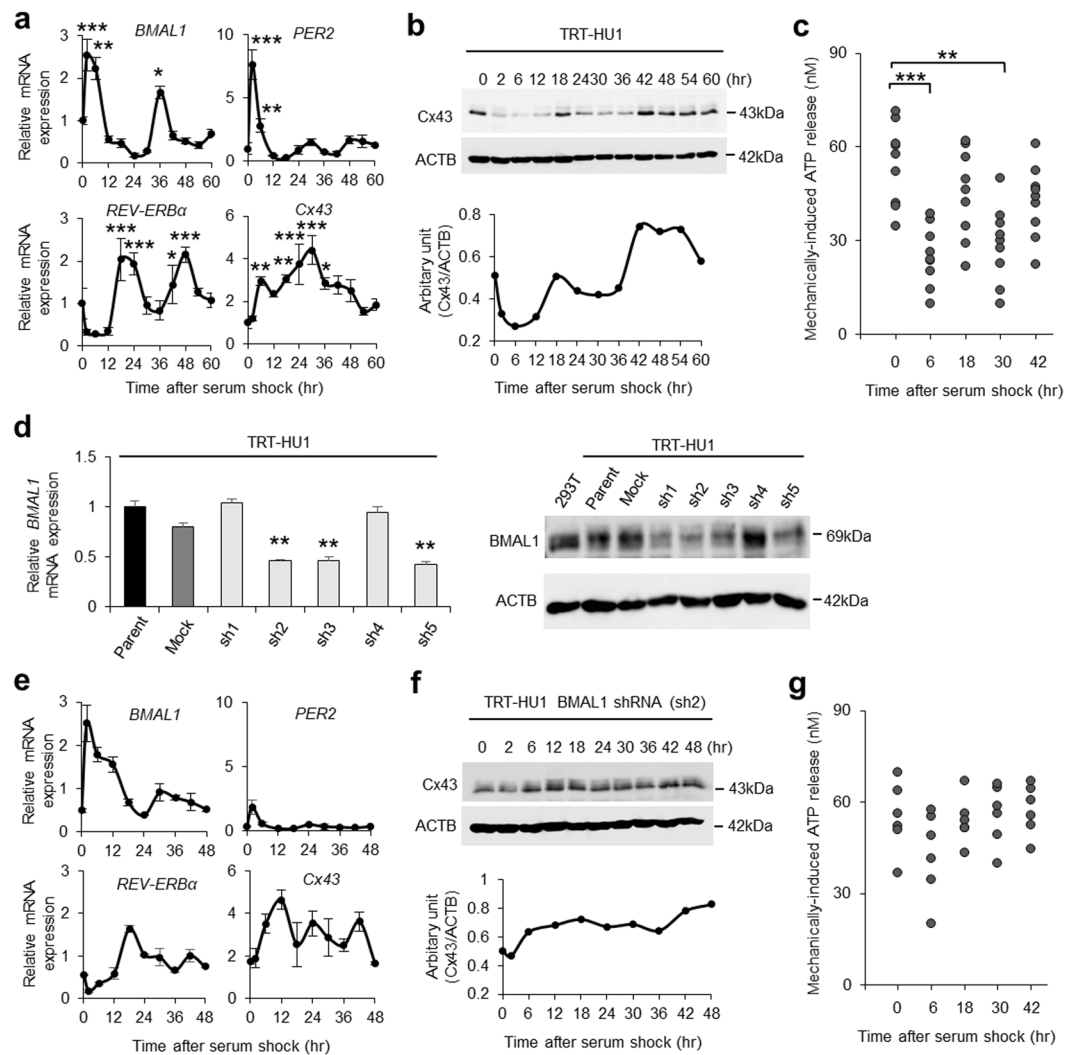
Figure 3. Oscillation of Cx43 and Clock gene expression in immortalized human urothelial cells. (a) Temporal variation of mRNA accumulation of clock genes and Cx43 mRNA levels in serum-shocked immortalized human urothelial cells (TRT-HU1). The major clock genes BMAL1 , PER2 , and REV-ERBα had circadian rhythms. * P < 0.05 , ** P < 0.01 and *** P < 0.001 vs. the nadir value (time 24 in BMAL1 , time 18 in PER2 , time 6 in REV-ERBα and time 0 in Cx43 ) by one-way ANOVA with Dunnett's post hoc test ( n = 3 ). The P -values with Cosinor analysis in Bmal1 , Per2 , Rev-erbα and Cx43 were 0.01, 0.0001, 0.002 and 0.09, respectively. (b) Representative immunoblots showing temporal changes in Cx43 protein levels in serum-shocked TRT-HU1 (Cosinor analysis, P = 0.006 ). Full-length blots are presented in Supplementary Fig. S12. (c) Temporal variation of mechanically induced ATP release in TRT-HU1 after serum-shock. ** P < 0.01 and *** P < 0.001 by one-way ANOVA with Dunnett's post hoc test ( n = 9 ). (d) Stable knockdown of BMAL1 in TRT-HU1 (sh1-sh5). ** P < 0.01 vs. mock by Student's t -test ( n = 3 ). Full-length blots are presented in Supplementary Fig. S12. (e) Temporal variation of mRNA accumulation of clock genes and Cx43 mRNA levels in serum-shocked sh2 TRT-HU1 (TRT-HU1 BMAL1 shRNA). (f) Representative immunoblots showing disturbed temporal changes in Cx43 protein levels in serum-shocked BMAL1 shRNA TRT-HU1. Full-length blots are presented in Supplementary Fig. S12. (g) Disturbed temporal variation of mechanically induced ATP release after serum-shocked sh2 TRT-HU1 ( n = 6 ). All error bars indicate s.e.m.
