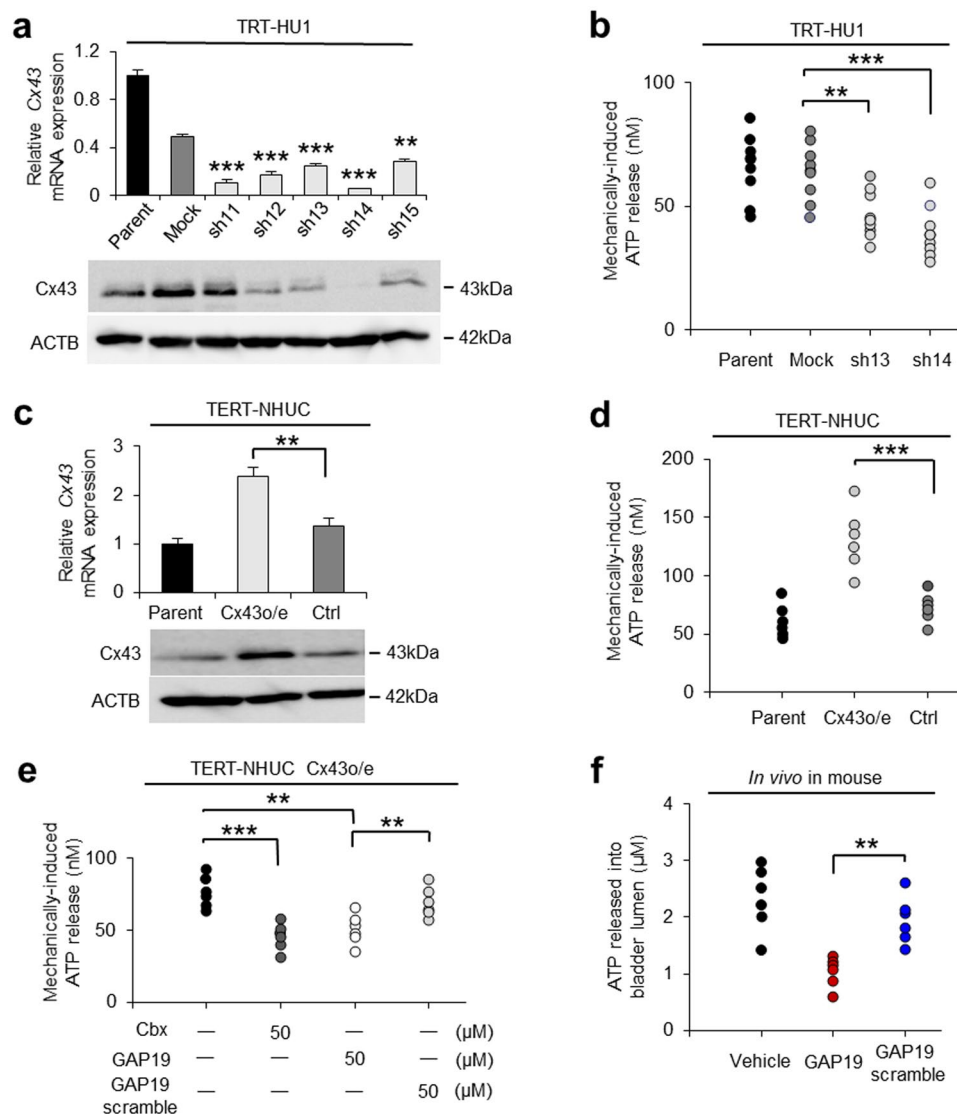
Figure 4. Mechanically induced ATP release via Cx43 hemichannels has diurnal variation. (a) Stable knockdown of Cx43 in TRT-HU1 (sh11-sh15). ^{**}P < 0.01 and ^{***}P < 0.001 vs. mock by Student's t -test ( n = 3 ). Full-length blots are presented in Supplementary Fig. S13. (b) Mechanically-induced ATP release was decreased in both sh13 and sh14 TRT-HU1. ^{**}P < 0.01 and ^{***}P < 0.001 by Student's t -test ( n = 9 ). (c) Cx43 -overexpression in TERT-NHUC ( Cx43 o/e TERT-NHUC). ^{**}P < 0.01 by Student's t -test ( n = 3 ). Full-length blots are presented in Supplementary Fig. S13. (d) Increased mechanically induced ATP release in Cx43 o/e TERT-NHUC. ^{***}P < 0.001 by Student's t -test ( n = 6 ). (e) Mechanically-induced ATP release in the presence of carbenoxolone and GAP19 peptide. Each reagent was used at 50 μM. ^{**}P < 0.001 by Student t -test ( n = 6 ). (f) The concentration of ATP release after bladder distention in the presence of GAP19 peptide and GAP19 scramble peptide in vivo in mice at ZT19. ^{**}P < 0.01 by Student's t -test ( n = 6 ). All error bars indicate s.e.m.
