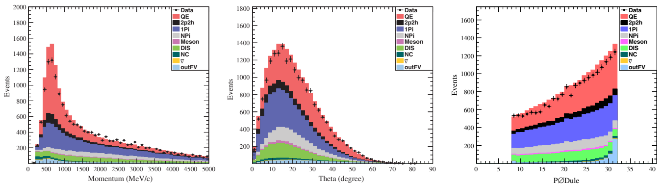
FIG. 3. FHC beam CCINC \nu_\mu event candidate distributions of the \mu^- momentum in MeV/c (left), the muon \theta_\mu angle in degrees (middle), and interaction vertex position by P \bar{\theta} Dule (right). Note backgrounds in the CCINC sample are the NC (dark green), \bar{\nu}_\mu induced events (yellow) and the out of fiducial volume events (light blue). There are negligible \bar{\nu}_\mu backgrounds (yellow) in the FHC sample.
