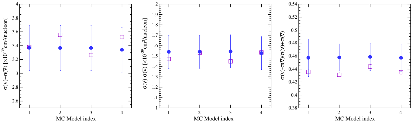
FIG. 8. Comparison of MC model 1–4 predictions, open squares with no errors bars, to data results, solid circles with error bars, in measurements of the cross section sum \Sigma = \sigma(\nu_\mu) + \sigma(\bar{\nu}_\mu) [left], difference \Delta = \sigma(\nu_\mu) - \sigma(\bar{\nu}_\mu) [middle] and asymmetry A = (\sigma(\nu_\mu) - \sigma(\bar{\nu}_\mu)) / (\sigma(\nu_\mu) + \sigma(\bar{\nu}_\mu)) [right].
