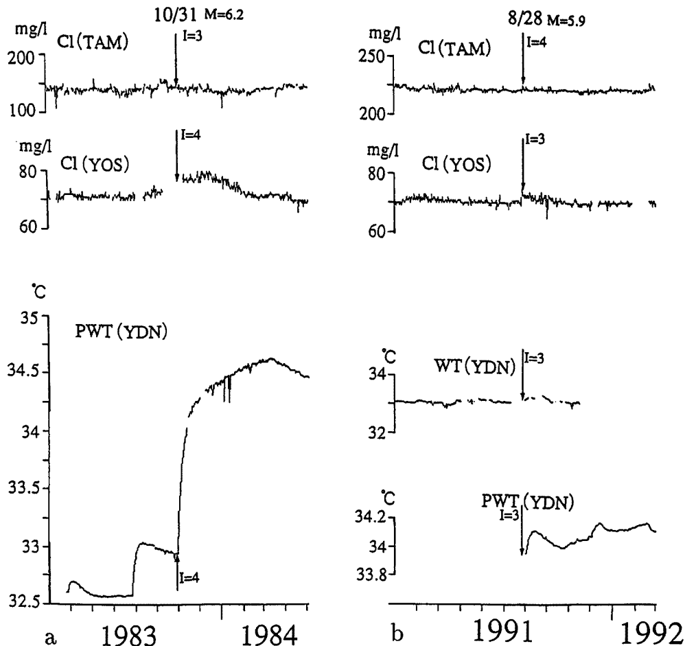
Fig. 8. Temporal variations of \text{Cl}^- concentration (Cl) and the groundwater temperature (WT, PWT) before and after the two large earthquakes in Tottori and Shimane Prefectures.
