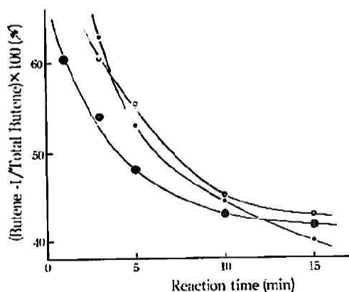
Fig. 8 The ratio of butene-1 to total butene vs. reaction time
