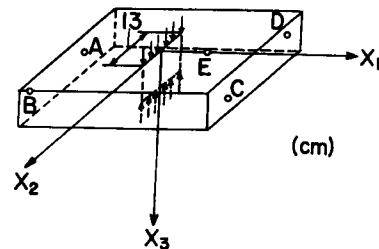
Fig. 4. Sketch of the split test, generating tensile cracks in the half space model specimen.
