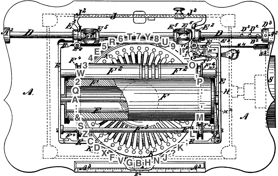
Fig. 11. Typebar basket of Sholes &amp; Glidden Type-Writer (top view)
