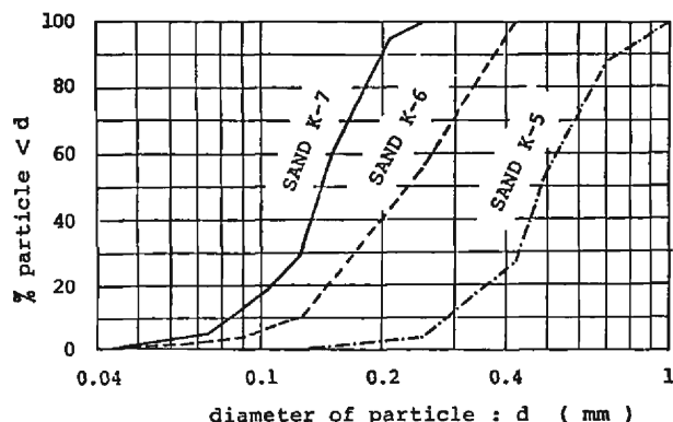
Fig. 1 Particle-size distribution.
