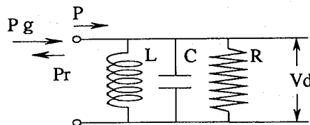
Fig. 1. Conventional untuned-type RF cavity using a quarter wavelength resonator.
