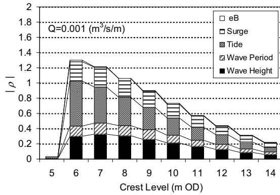
Fig. 4 Annual failure probability of sloping seawall by Level III analysis
