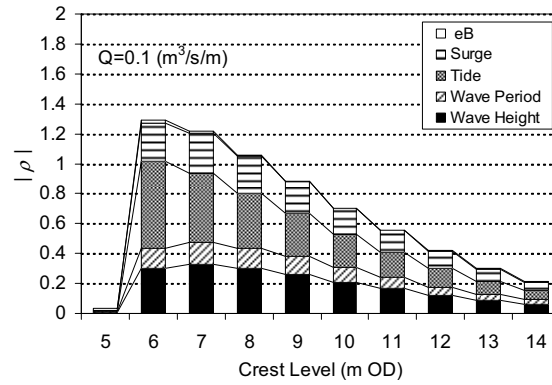
Fig. 6 Spearman's rank correlation coefficient for the case of sloping seawall
