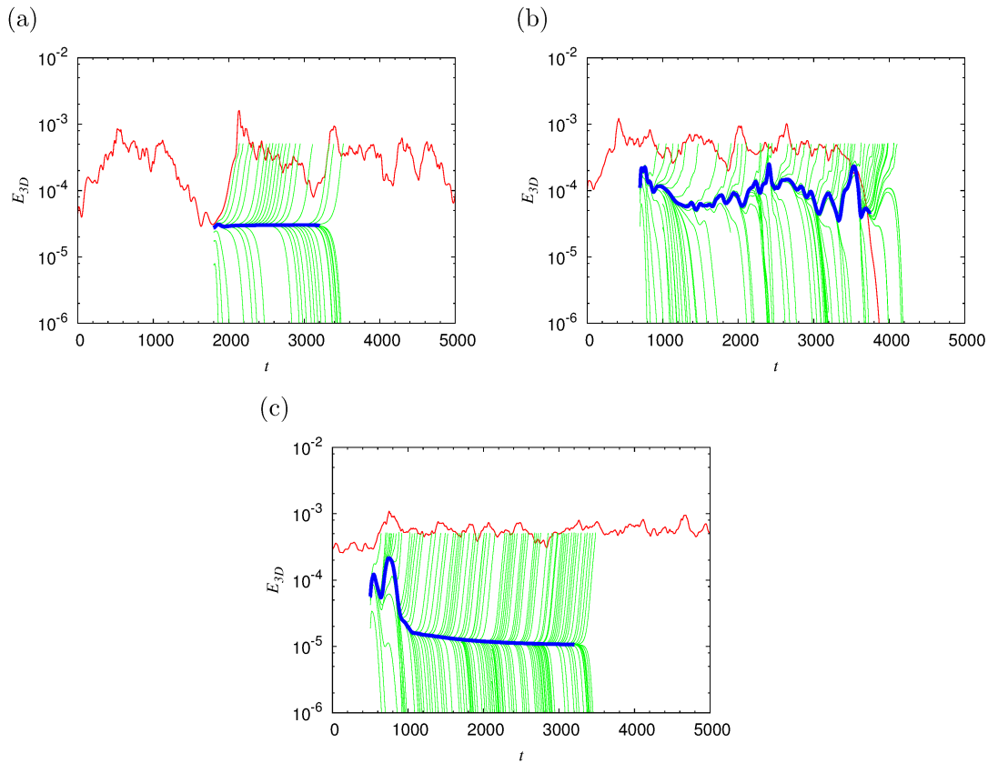
図 1: (Thin) Time evolution of the three-dimensional energy E_{3D} for (a) L_x = 2\pi , (b) L_x = 4\pi , (c) L_x = 8\pi . (Grey) Trajectories that grow to turbulence or laminarize. (Bold) Edge trajectory.
