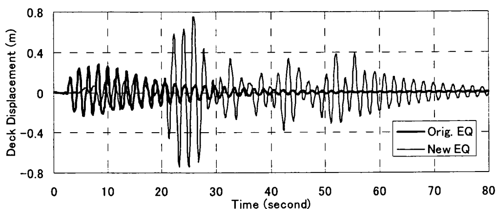
Figure 4-15. Deck displacement time history of the Tempozan Bridge model under original (scaled Parkfield NE) and new (Type 1-III-3) design earthquakes in the lateral direction (First mode natural period T = 1.79 second)
