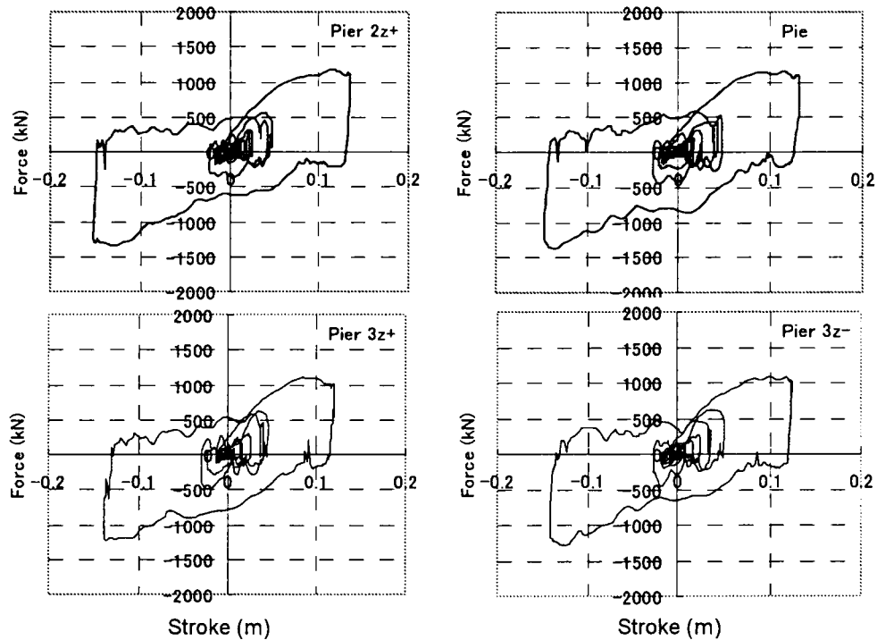
Figure D-17. PNS damper plus bearing hysteretic loop at pier2 and pier3 (Gebze, incidence angle 45^\circ )
