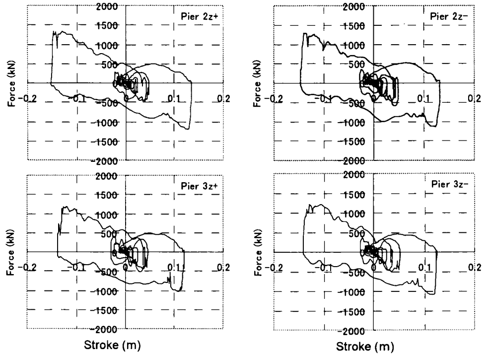
Figure D-16. PNS damper hysteretic loop at pier2 and pier3 (Gebze, incidence angle 45^\circ )
