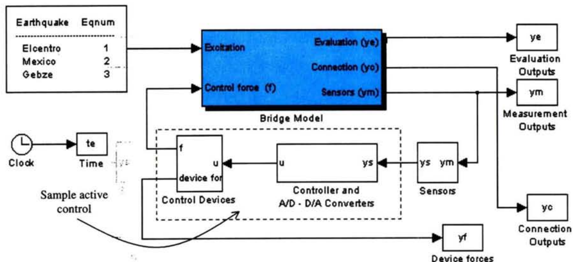
Figure D-1. Original SIMULINK block diagram in the benchmark problem with sample active control
