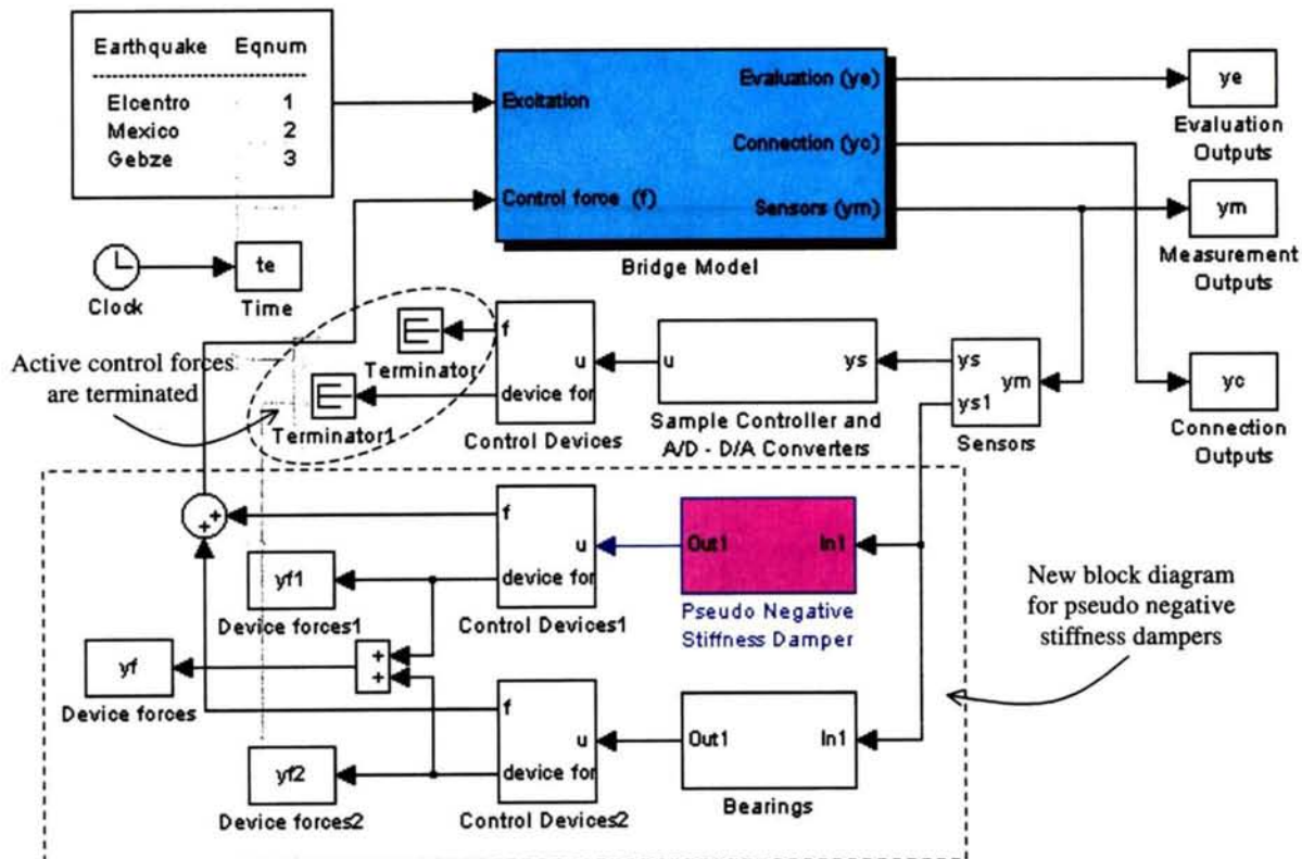
Figure D-2. Modified SIMULINK block diagram for application of pseudo negative stiffness damper
