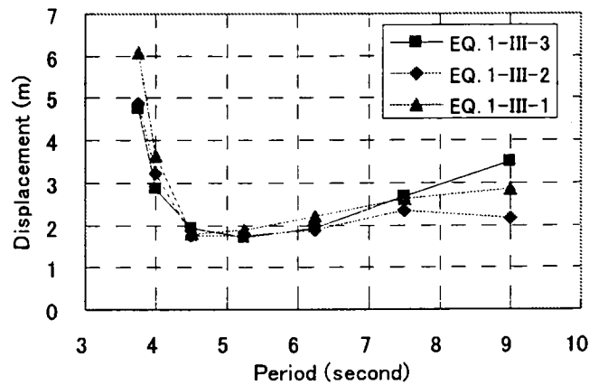
Figure 4-19. Displacement response, damping ratio \zeta = 20\% (Type 1-III-3, 1-III-2, & 1-III-1: artificial ground accelerations used for design in Japan for soft soil condition)
