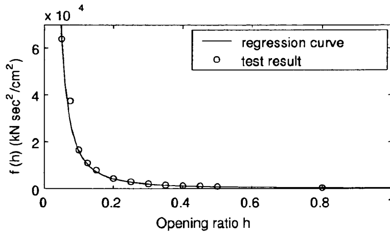
Figure E-3. Regression curve of the coefficient of the square of relative velocity
