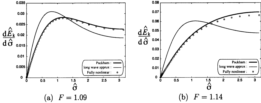
Fig.4 Comparison of the kinetic energy density d\hat{E}_k/d\hat{\sigma} . F = c/\sqrt{gh} : the Froude number, thin line : long wave approximation, thick line : Packham's approximation and circle \circ : fully nonlinear solution.
