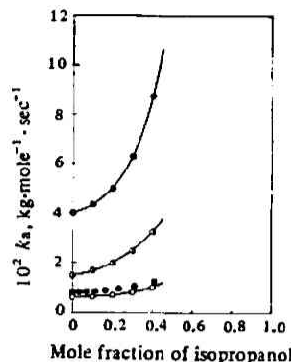
Fig. 2 Variation of the rate constants for the decomposition of diacetone alcohol in aqueous isopropanol at 1 atm Åkerlöf (9) : \otimes ...25°C This work: \circ ...20.00°C, \odot ...30.00°C, \bullet ...40.00°C
