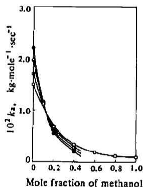
Fig. 1 Variation of the rate constants for the decomposition of diacetone alcohol in aqueous methanol at 1 atm Åkerlöf (9) : \otimes ...25°C Murphy (10) : \circ ...20°C, \circ ...30°C LaMer et al. (11) : \odot ...30°C This work: \circ ...20.00°C, \odot ...30.00°C, \bullet ...40.00°C
