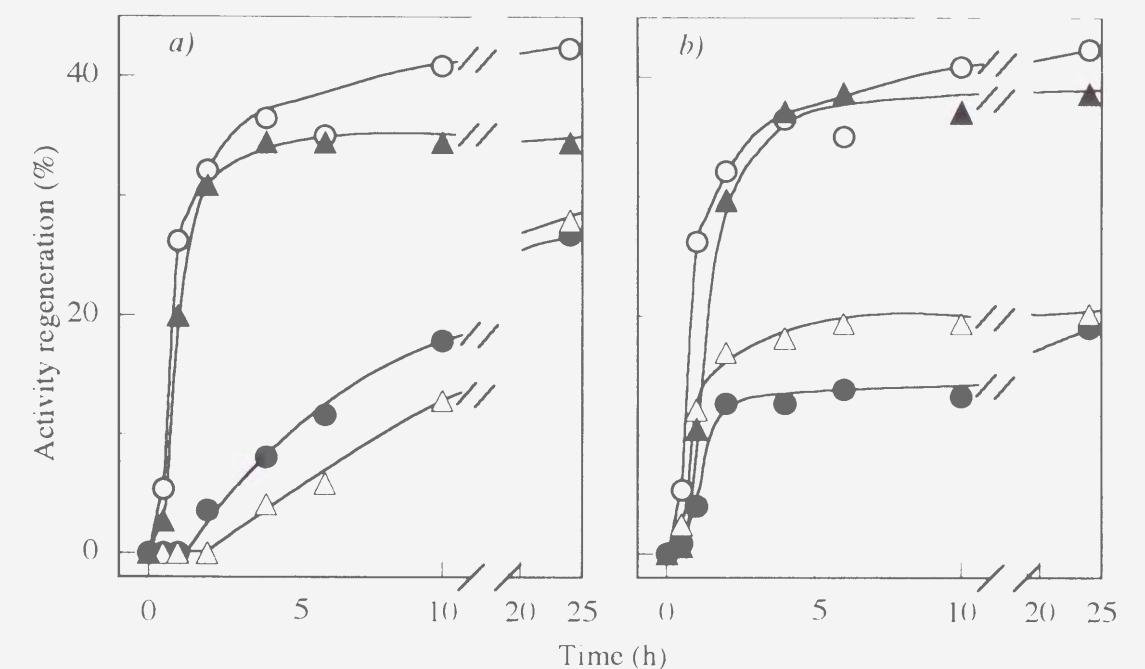
Fig. 8. Recovery of the activity on air oxidation in the absence of glutathione.
