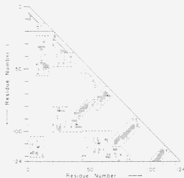
Fig. 3. Contact map of RNase S. Each point of the map represents presence (square) or absence (no marking) of a contact between amino acid residues i and j . Contacts between residues are omitted from the figure whenever |i-j| < 4 . (From ref. 59)
