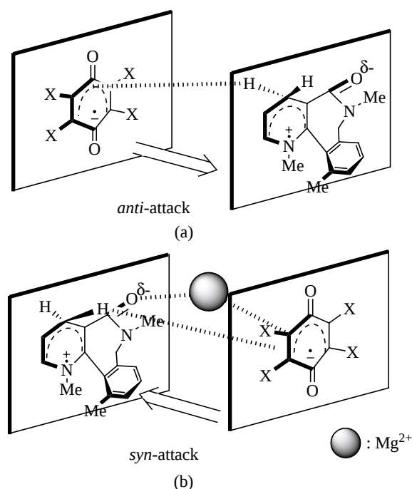
Figure 1. Pre-association complex between NAD(P)H model and quinone without \text{Mg}^{2+} (a) and with \text{Mg}^{2+} (b) from initial electron transfer.
