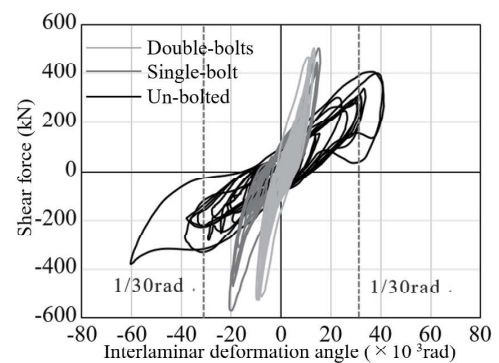
Figure 2. Interlaminar deformation angle relationship of shear force under 135% excitation of BSL wave (1st layer).
