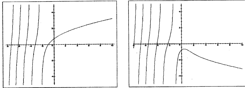
Figure 3.4: Left part: function -A'_i(x)/A_i(x) . Right part: function -B'_i(x)/B_i(x)
