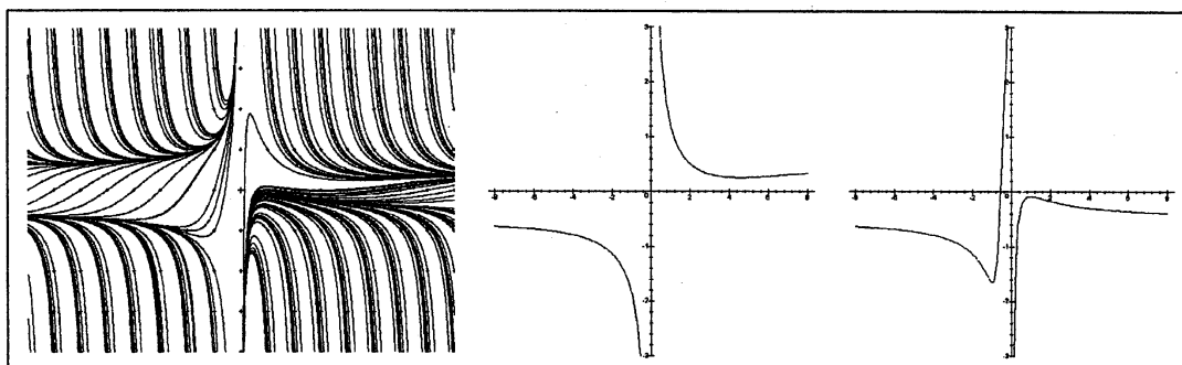
Whittaker's equation for \kappa = 1 and \mu = 2 . Function M'_{1,1}(x)/M_{1,1}(x) . Function W'_{1,1}(x)/W_{1,1}(x)
