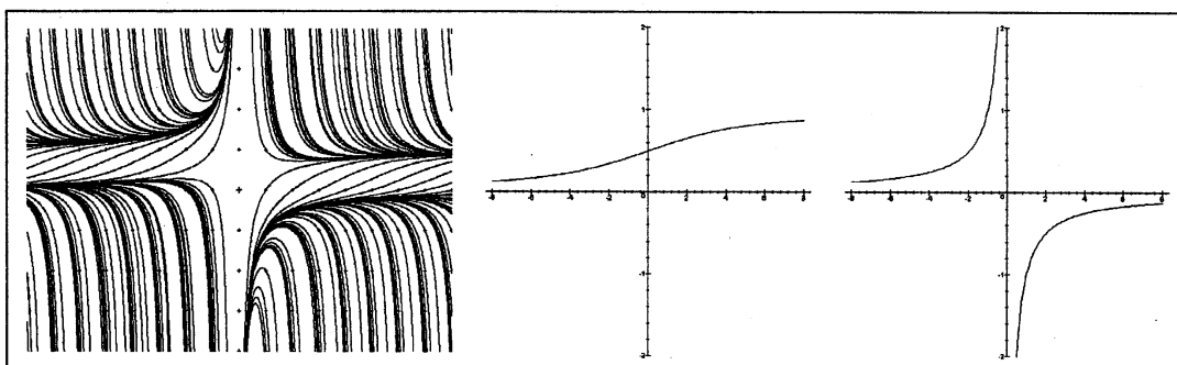
Kummer's equation for a = 1 and b = 2 . Function M'(1, 2, x)/M(1, 2, x) . Function U'(1, 2, x)/U(1, 2, x)
