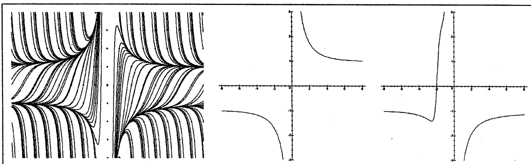
Modified Bessel's equation for v = 3 . Function I'_3(x)/I_3(x) . Function K'_3(x)/K_3(x)
