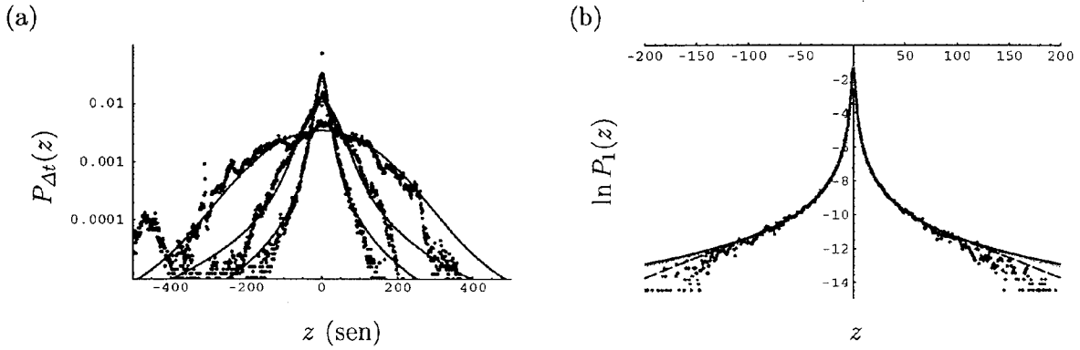
Figure 2: (a) Empirical density functions P_{\Delta t}(z) for sampling intervals of \Delta t = 2^{15}, 2^{18}, 2^{21} seconds (dots) and the corresponding stable density functions (lines, \alpha = 1.451, 1.588, 1.900 and \gamma\Delta t = 23.86, 184.5, 4276 ) estimated by the maximum log likelihood. (b) Comparison the shapes of P_1^{ELJ}(z) , P_1^G(z) , the stable density and the simulation's empirical density of ELJ when \Delta s = 1 . b = 3 , Q = 2 , N = 10000 .
