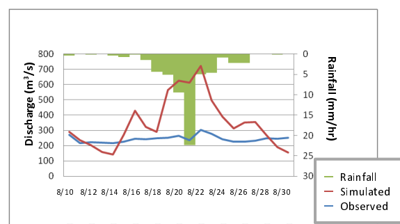
Fig.7 Discharge rates at Fushiguro
