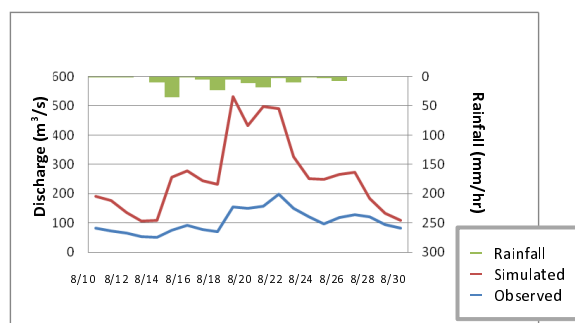
Fig.5 Discharge rates at Fushiguro
