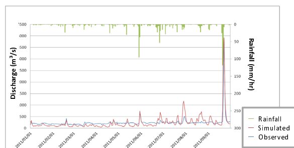
Fig.9 Discharge rates at Iwanuma in 2011
