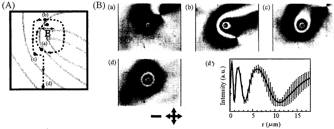
Figure 1: Formation of triple ring-like wall induced by an orbiting trajectory of beam spot illustrated in (A) around a +1/2 wedge disclination. The corresponding snapshots are inserted in (B). (a)-(c) The snapshots showing the single, double and triple wall structure respectively. (d) Triple ring-like wall structure averaged for 6 seconds. (d') Averaged radial intensity profile of (d) with error bars every four data point. When the laser irradiation is shut off the multiple ring structure dissolves over a period of a few seconds. Scale bar represents 10 \mu\text{m} . The crossed black double-head arrow represents the direction of crossed Nicols.
