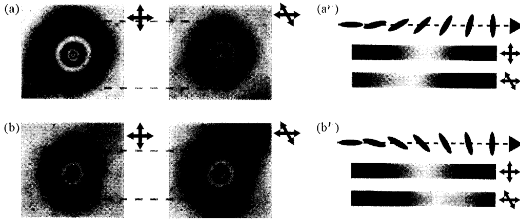
Figure 2: (a) Shrink and (b) spread of the multiple wall structure observed by an analyzer rotation. Primed figures are the schematic representation of the director rotation and the transmitted light intensity along the radial direction. The double-head arrow is the direction of analyzer and polarizer.
