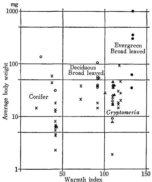
Fig. 4. Average body weight and warmth index.
