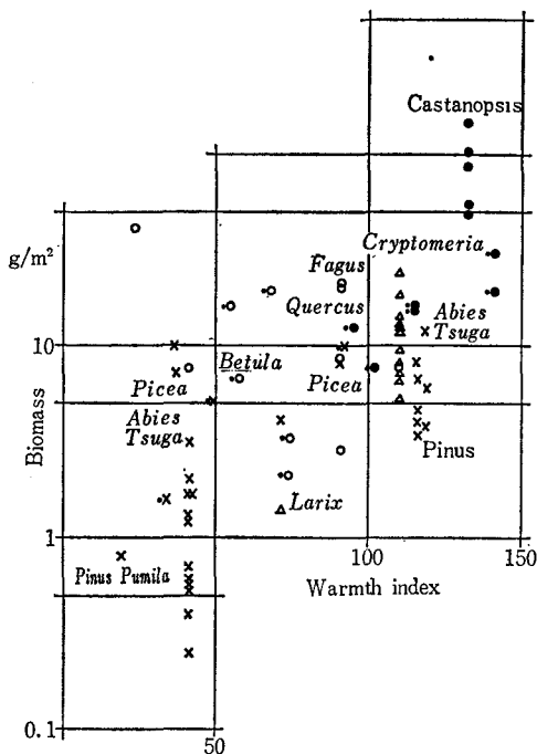
Fig. 3. Biomasses in relation to warmth index.
