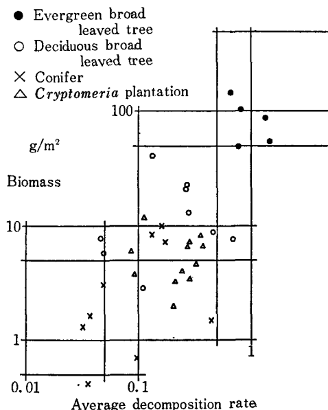
Fig. 9. Relation between average decomposition rates and biomasses of macro animals.
