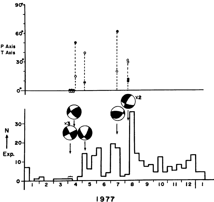
Fig. 6(b). Relation between the volcanic activity and the focal mechanism of A type earthquakes. Angles of P and T axes are measured from horizontal plane. Black quadrants are of compression. The numbers near the mechanism diagrams denote the number of earthquakes composited.
