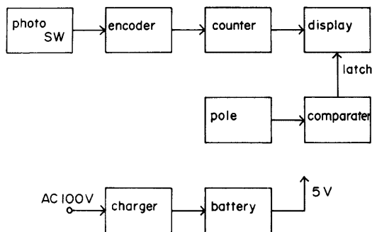
Fig. 2. Block diagram of the digital water level gauge.
