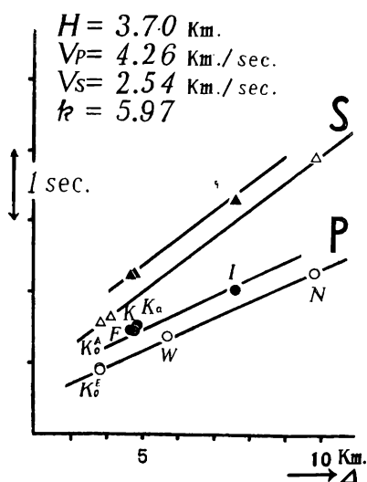
Fig. 3. Time-distance curves. (No. 250)
