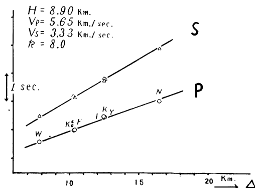
Fig. 4. Time-distance curves. (No. 228)
