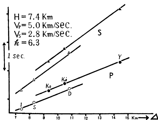
Fig. 2. Time-distance curves. (No. 140)
