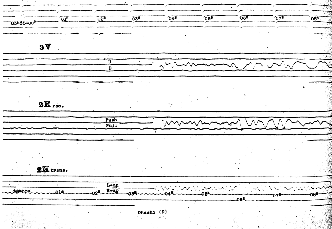
Fig. 10. Seismogram recorded by the R_2 -seismometers in an explosion seismic observation. (at Ohashi-station, May, 3rd, 1954, 03h35m, Kamaishi-explosion.)
