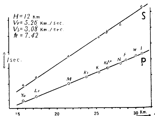
Fig. 5. Time-distance curves. (No. 247)
