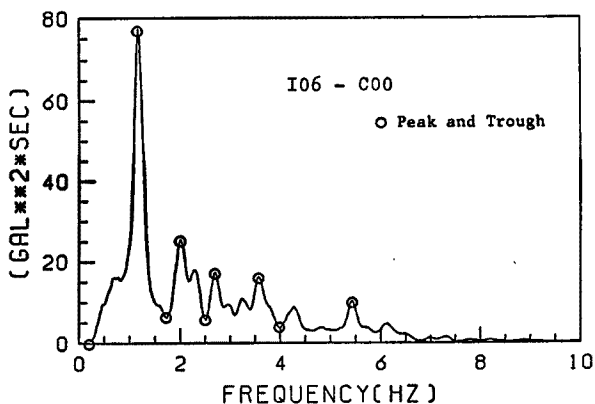
Fig. 5 Stationary Cross Spectra of SMART-1 Array Accelerograms.
