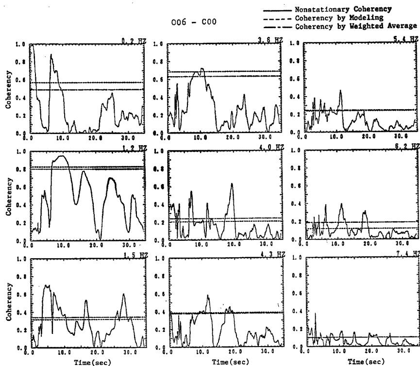
Fig. 10 Nonstationary Coherency and Representative Values by Modeling and Weighted Average (006-C00).
