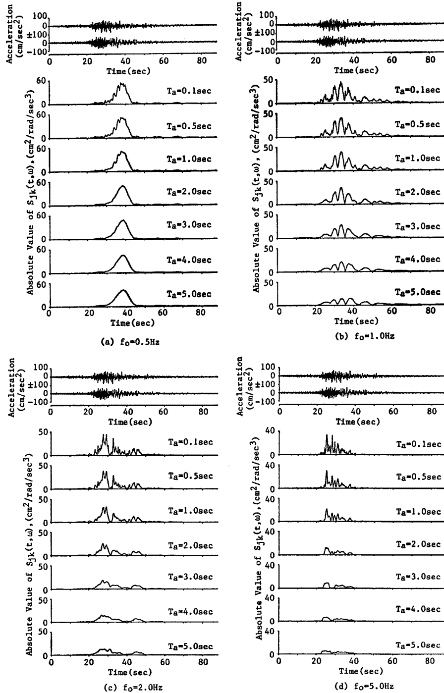
Fig. 2 Amplitude of Nonstationary Cross Spectra of Hachinohe EW and NS Components. ( h_0=0.05 )
