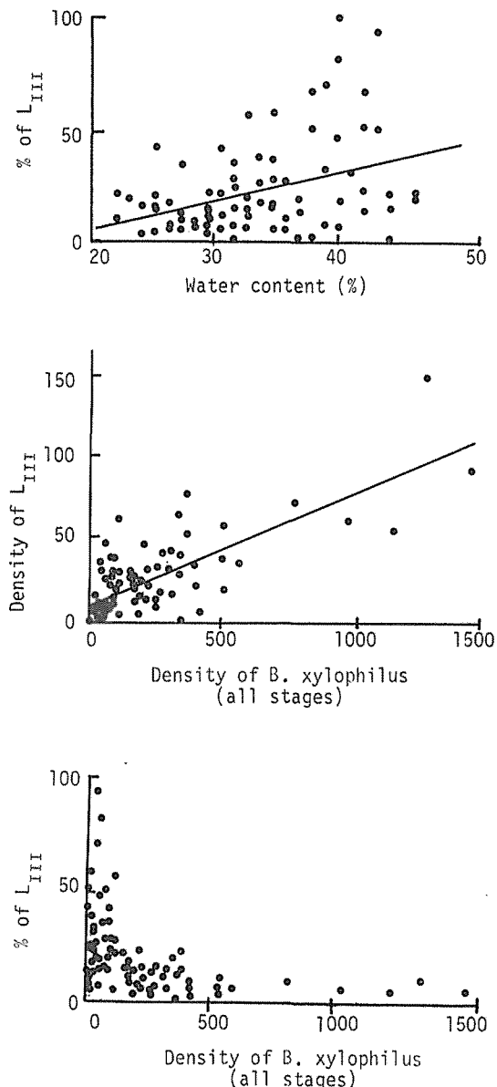
Fig. 8 The relationships in November between the ratio of dispersal 3rd stage larvae ( L_{III} ) of B. xylophilus and water content of the log examined (top), between the density of total population of B. xylophilus and that of L_{III} (middle), and between the density of total population of B. xylophilus and the ratio of L_{III} (bottom).
