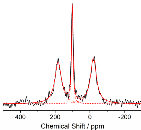
Figure 5. Spectral decomposition of the ^{207}\text{Pb} MAS spectrum of \beta^+ - \text{PbSnF}_4 at 80^\circ\text{C} (the black line) by three Lorentzian lineshapes (the red dotted lines). The sum of the three Lorentzian lineshapes is given by the red solid line. For quantitative analysis, the pulse-repetition time 13 s was set to be much longer than the spin-lattice relaxation times of the three signals (Pb-a: ca. 1.2 s, Pb-b: ca. 1.6s, and Pb-c: ca. 1.9 s).
