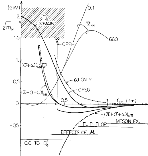
Fig. 1. Nucleon-nucleon ( NN ) potentials in the ^1S_0 state and illustration of the regions where the various processes explained in the text are effective. OPEH (OPEH) is a realistic potential with the OPEH-tail and the Gaussian soft core (hard core). The solid line denoted by (\pi + \sigma + \omega)_{NN} is the meson-theoretical potential given by Eq. (1) and the parts from (\sigma + \omega) and \omega only are shown by the dotted lines. The dashed line is the corresponding potential in the N\bar{N} system. The shaded area indicates the domain of possible appearance of exotic dibaryon states D_0^+ . The lines denoted by \Psi_{NN} is an example of the relative wave function with one radial node at E_{Lab}^{NN} = 0.1 and 660 MeV (in arbitrary unit). 15b) O.C. is the abbreviation to orthogonality condition.
