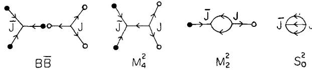
Fig. 5. A series of boson-like states, \mathcal{M} : M_4^2 , M_2^2 and S_0^2 are exotic baryonium states produced by connecting q and \bar{q} ends successively in B\bar{B} . 8)
