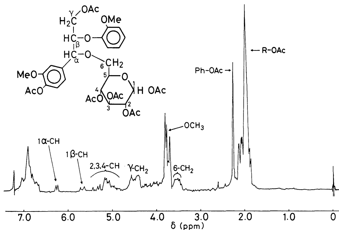
Fig. 11. NMR spectrum of guaiacylglycerol- \alpha -[6'- O -(1',2',3',4'-tetra- O -acetyl- D -glucose)]- \beta -guaiacyl ether diacetate in \text{CDCl}_3
