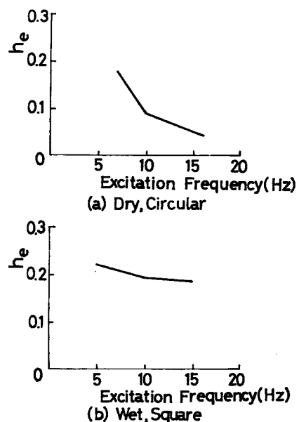
Fig. 9 Hysteresis damping factors h_e .
